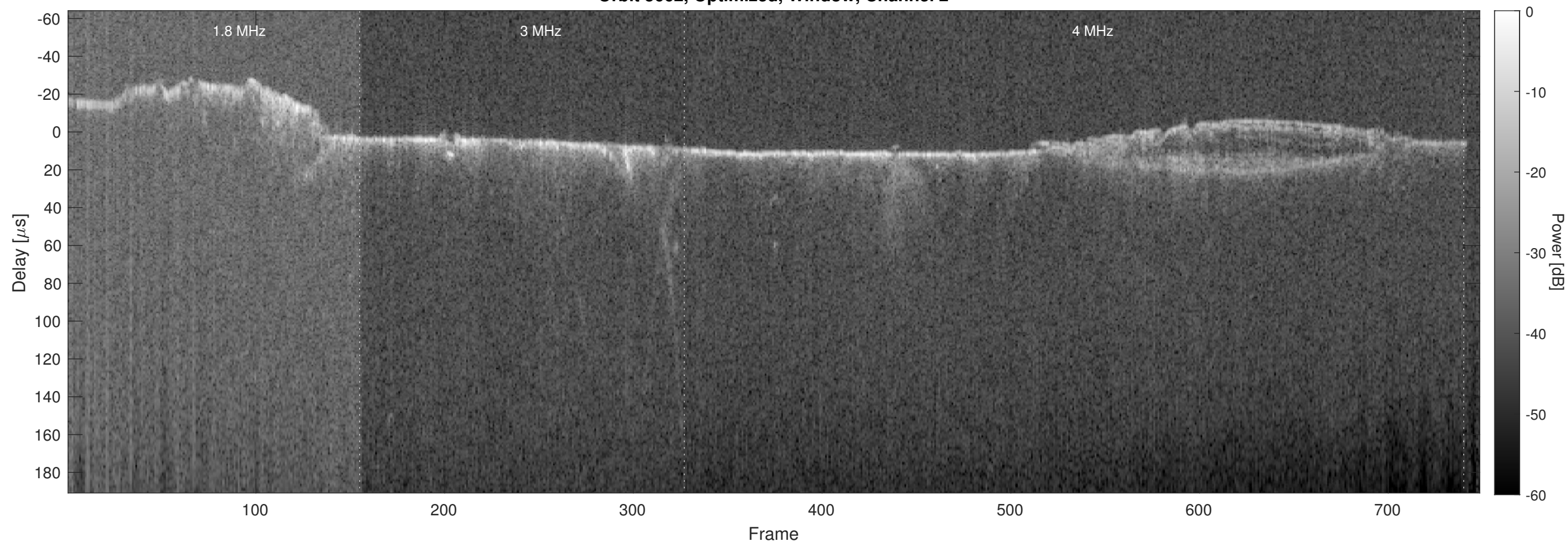
Orbit 5662, Optimized, Window, Channel 2
