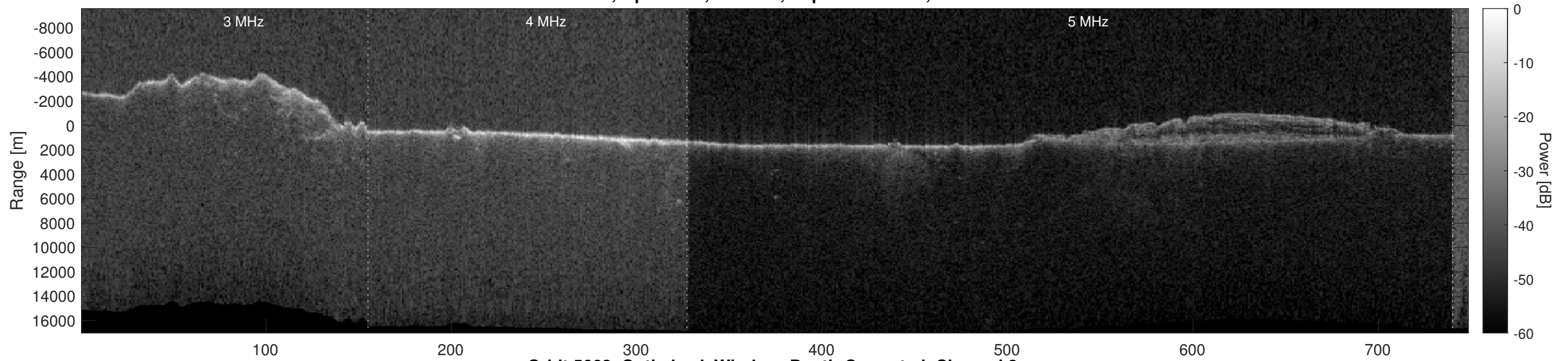
Orbit 5662, Optimized, Window, Depth-Corrected, Channel 2
