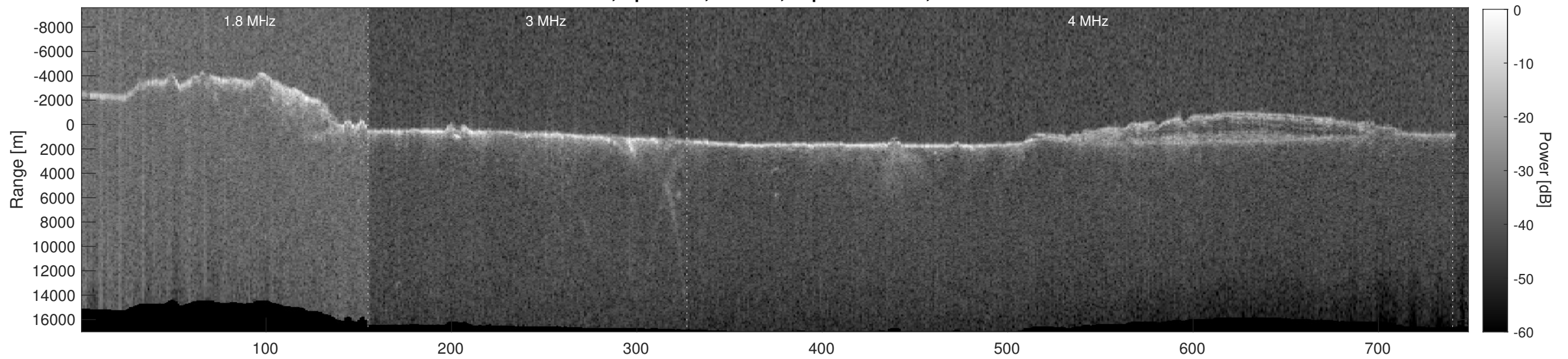
Orbit 5662, Depth-Corrected Cluttergram
