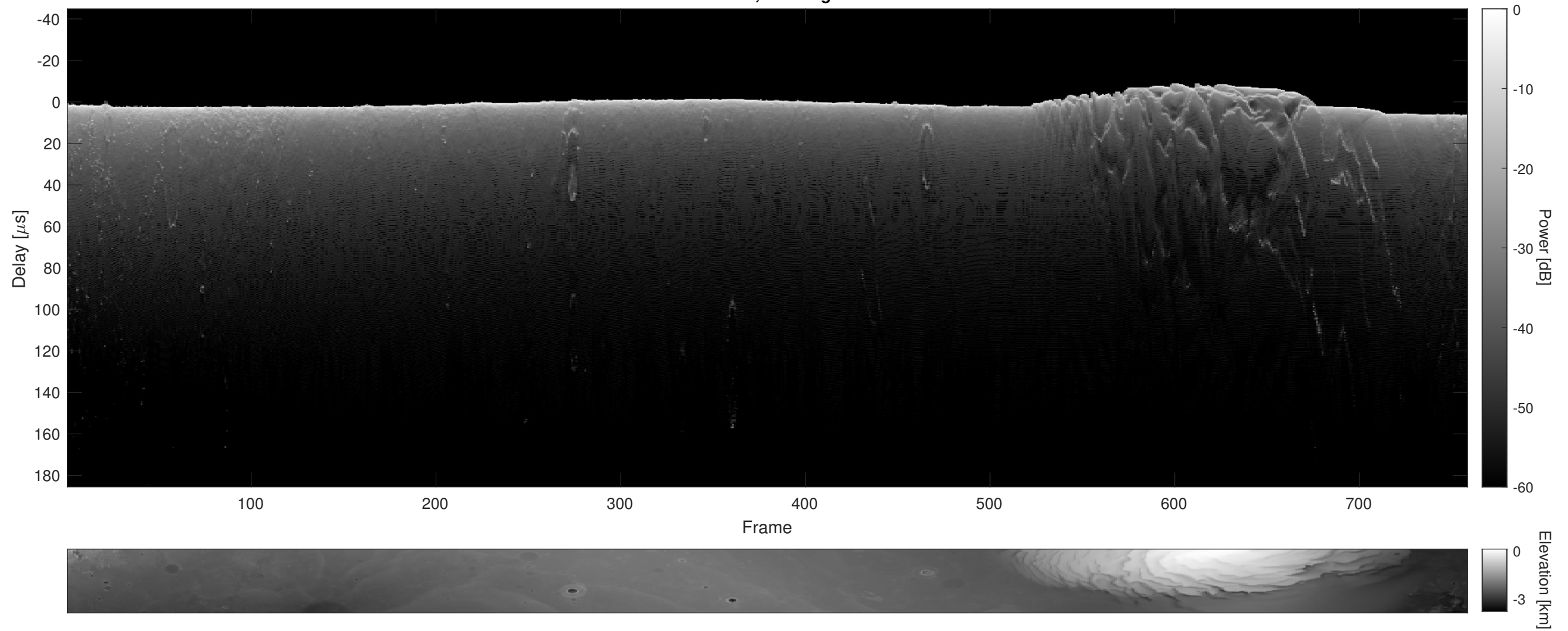
Orbit 5664, Cluttergram
