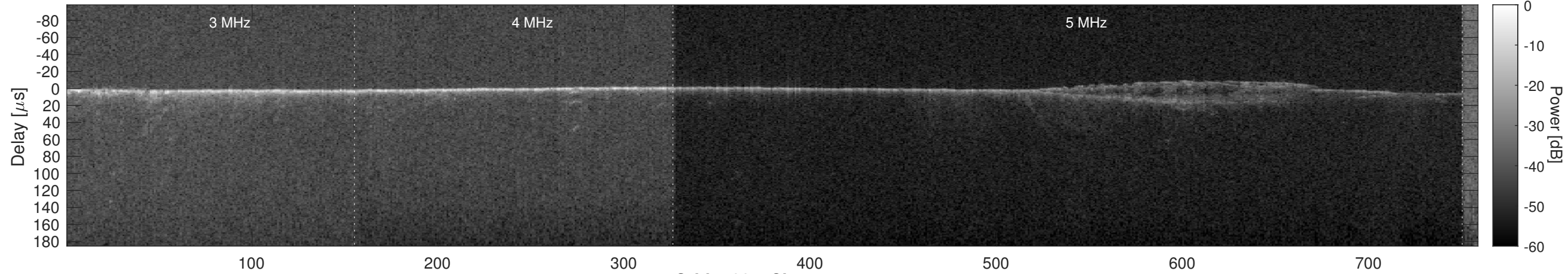
Orbit 5664, Cluttergram
