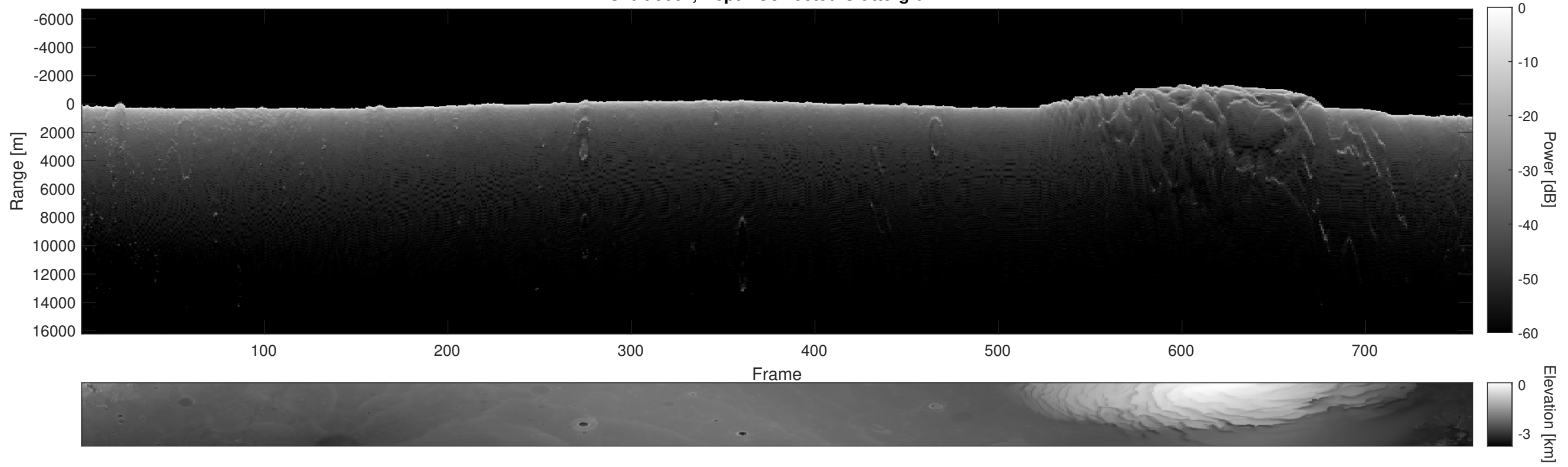
Orbit 5664, Depth-Corrected Cluttergram
