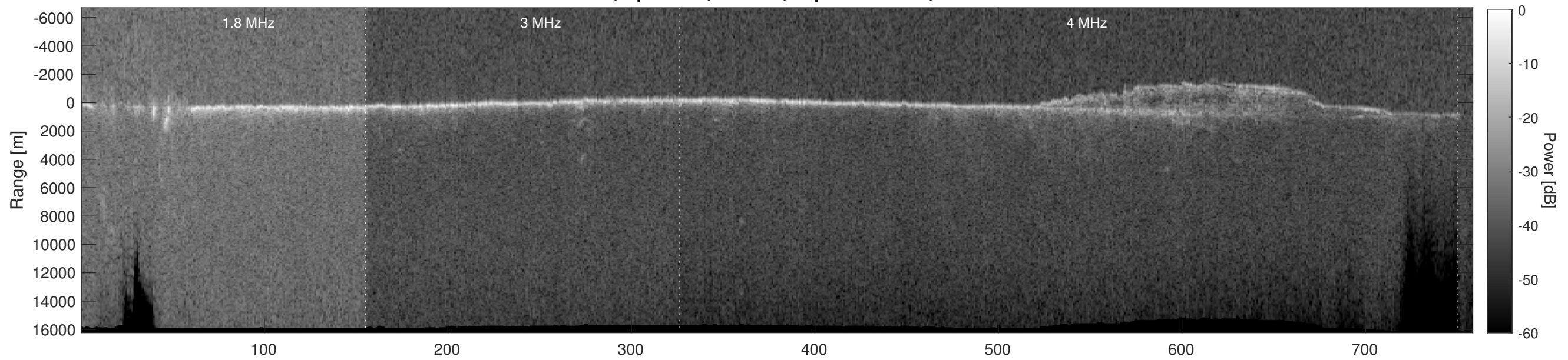
Orbit 5664, Depth-Corrected Cluttergram
