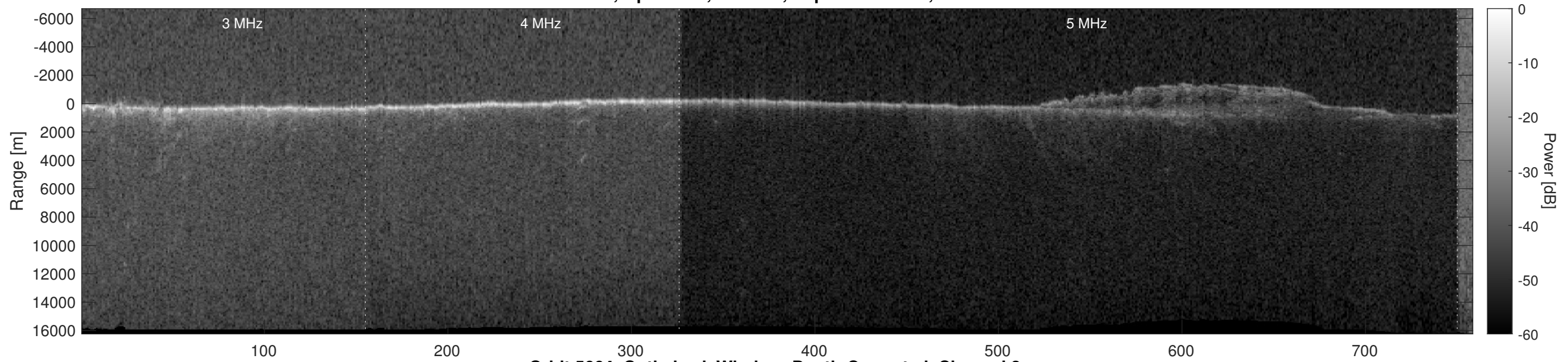
Orbit 5664, Optimized, Window, Depth-Corrected, Channel 2
