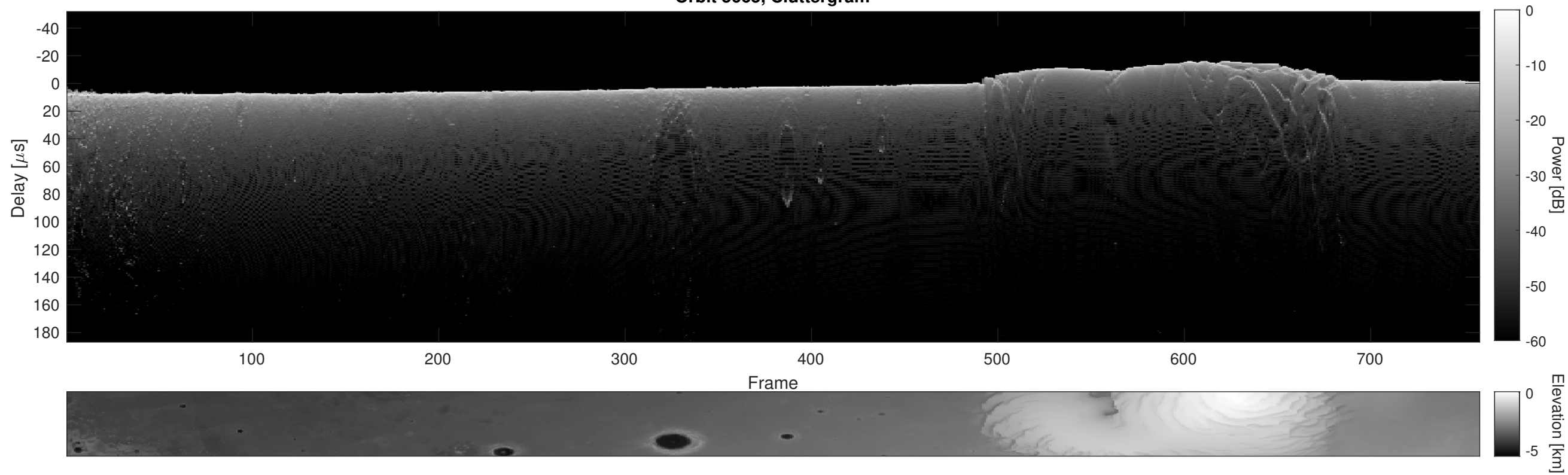
Orbit 5665, Cluttergram
