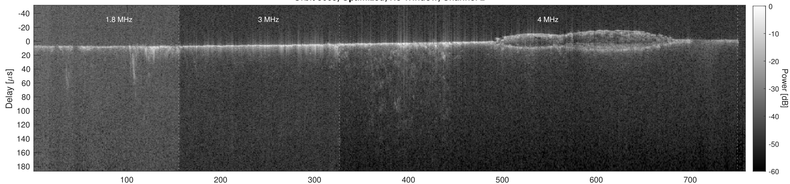
Orbit 5665, Cluttergram
