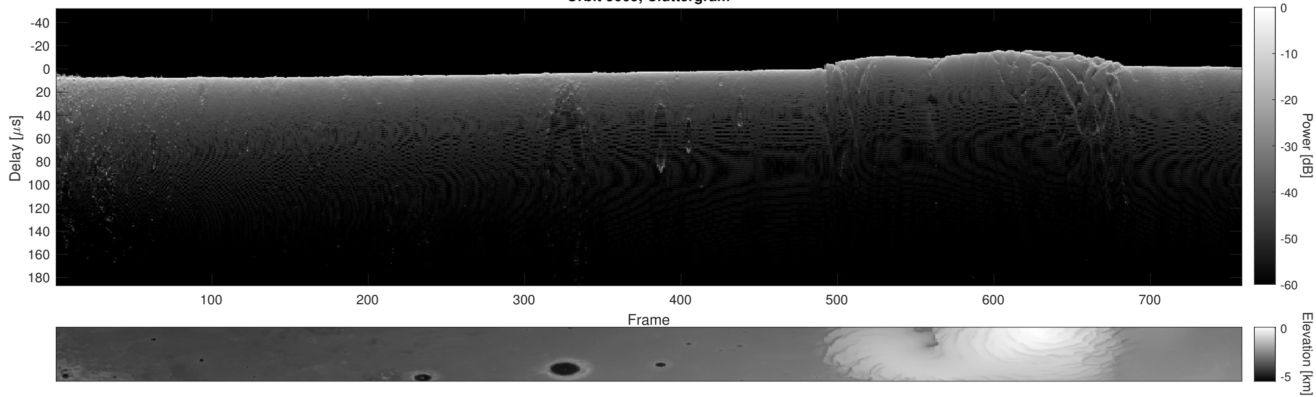
Orbit 5665, Cluttergram
