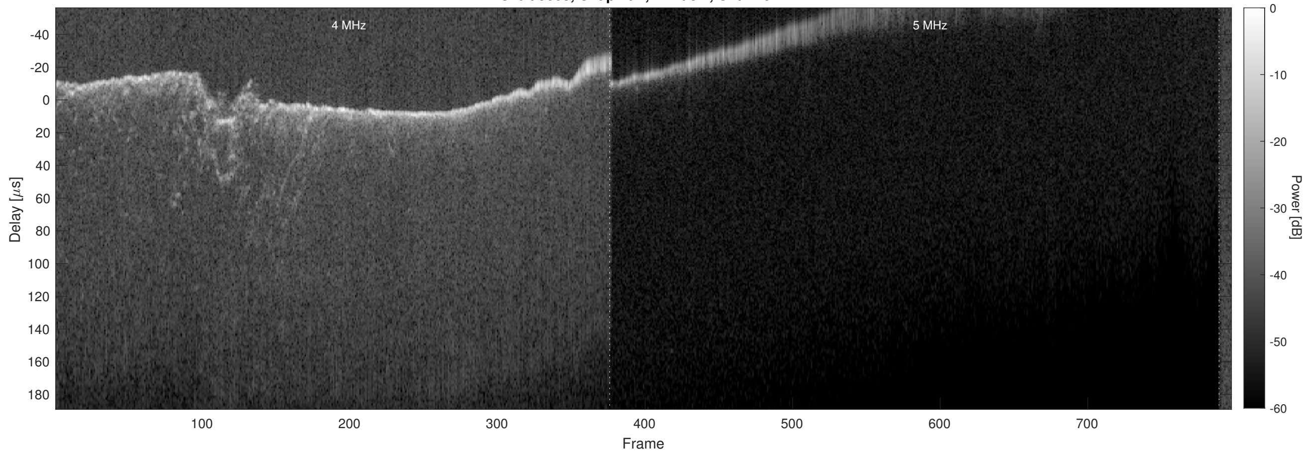
Orbit 5668, Chapman, Window, Channel 2
