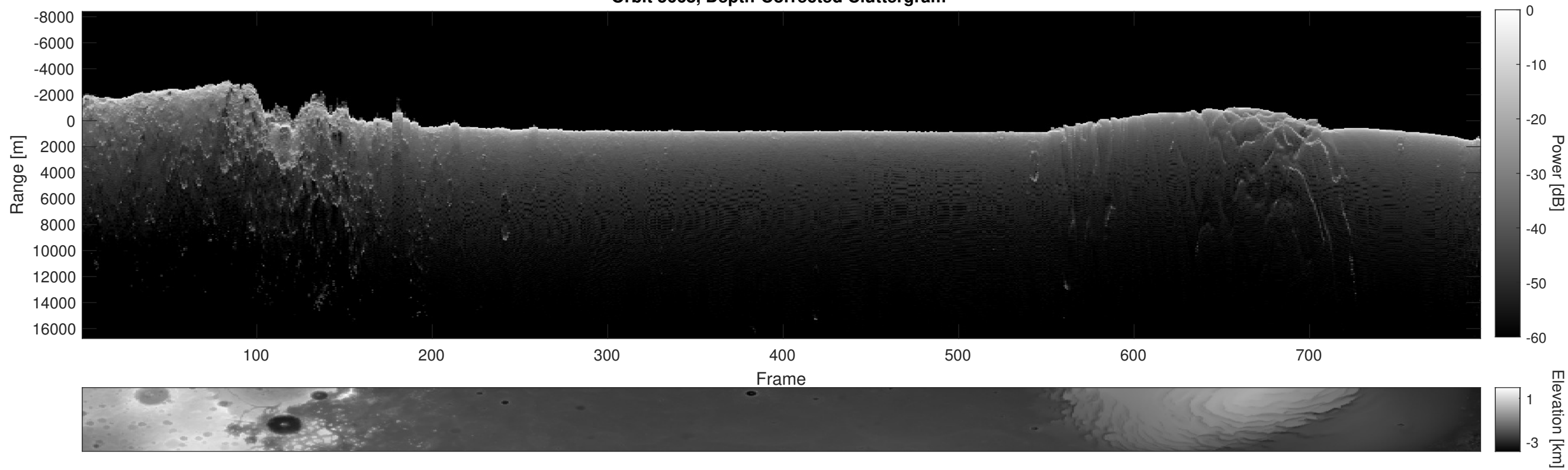
Orbit 5668, Depth-Corrected Cluttergram
