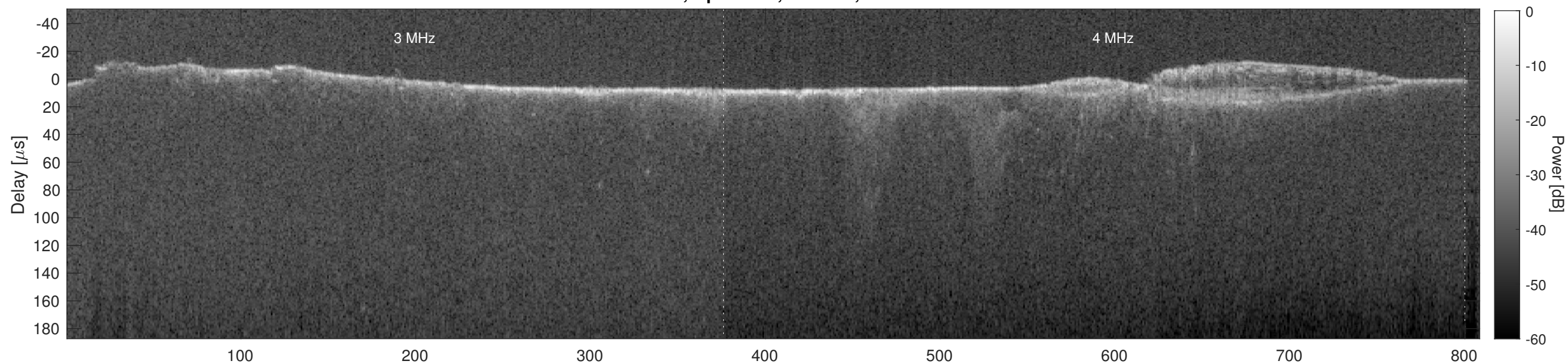
Orbit 5669, Cluttergram
