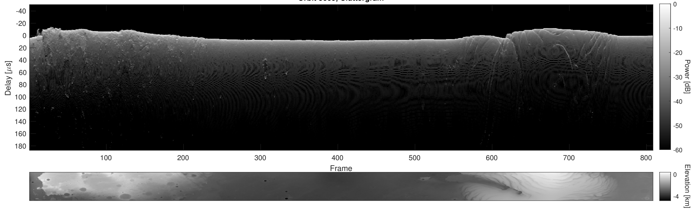
Orbit 5669, Cluttergram
