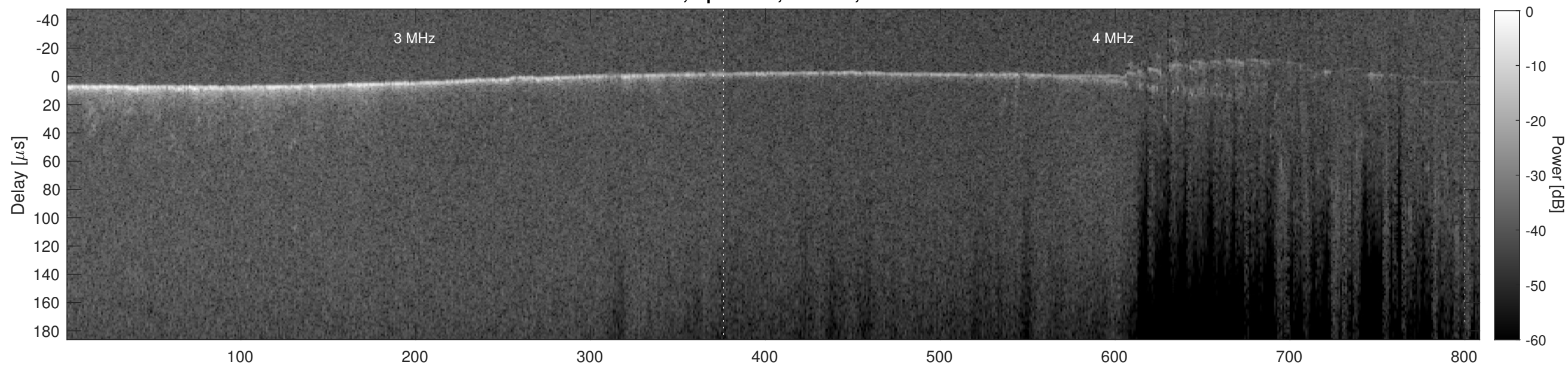
Orbit 5671, Cluttergram
