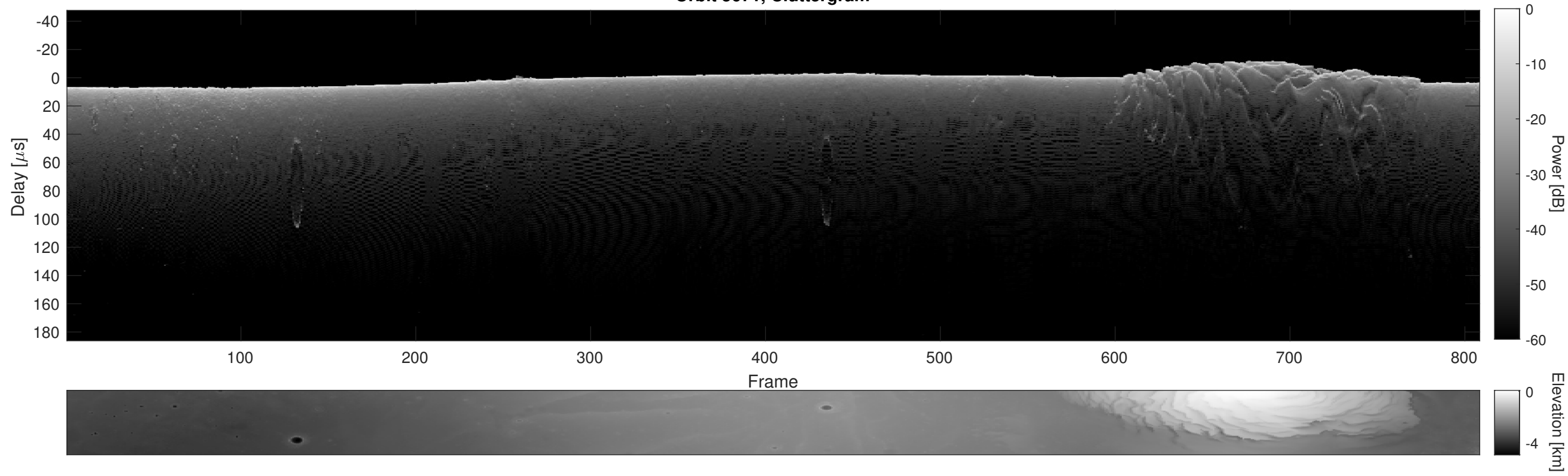
Orbit 5671, Cluttergram
