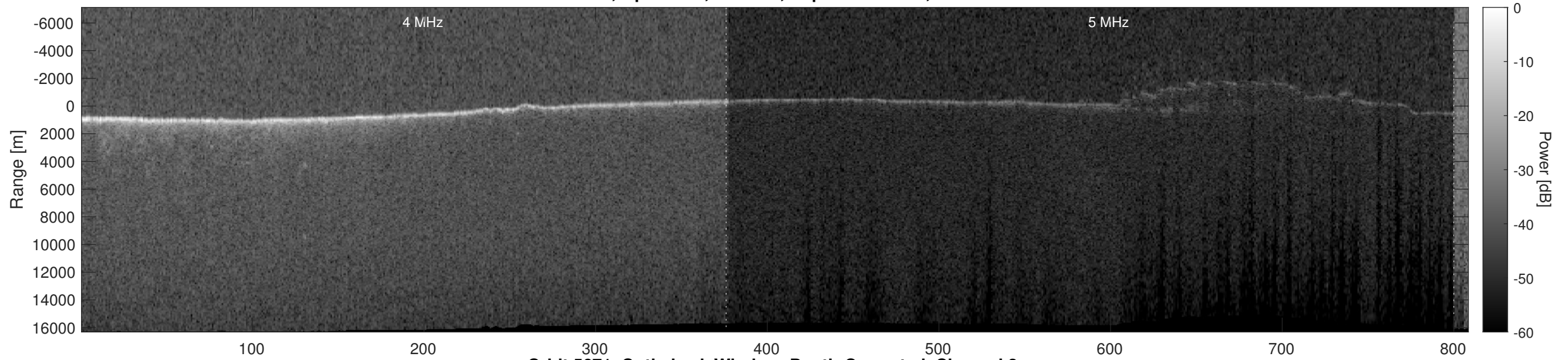
Orbit 5671, Optimized, Window, Depth-Corrected, Channel 2
