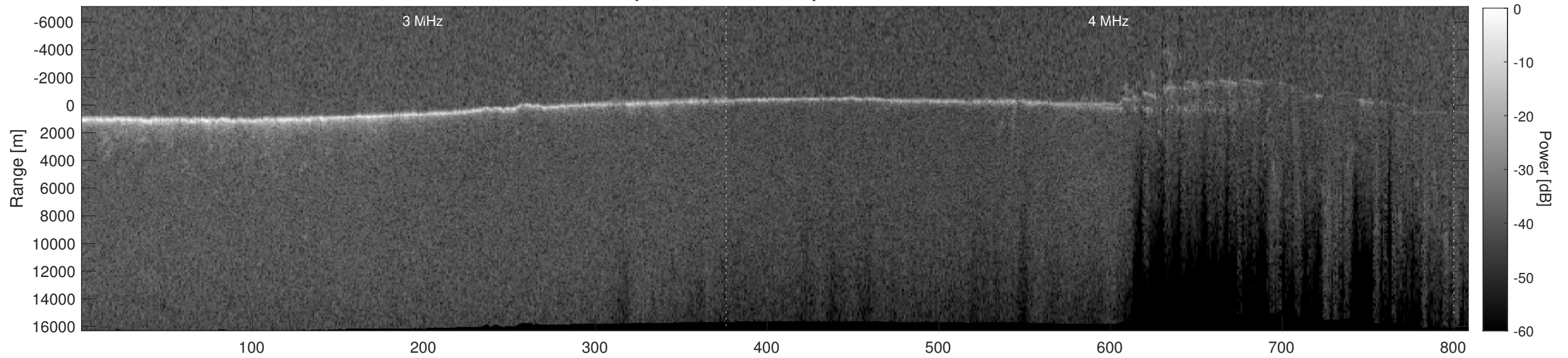
Orbit 5671, Depth-Corrected Cluttergram
