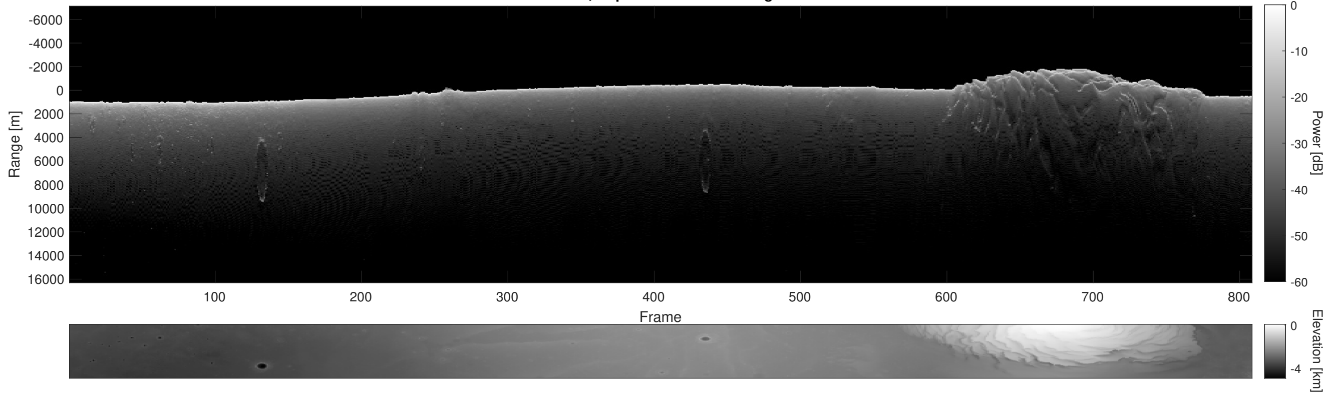
Orbit 5671, Depth-Corrected Cluttergram
