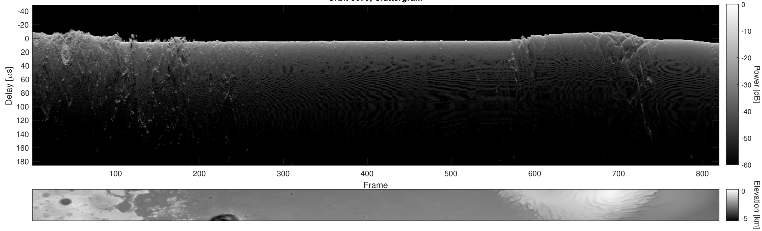
Orbit 5679, Cluttergram
