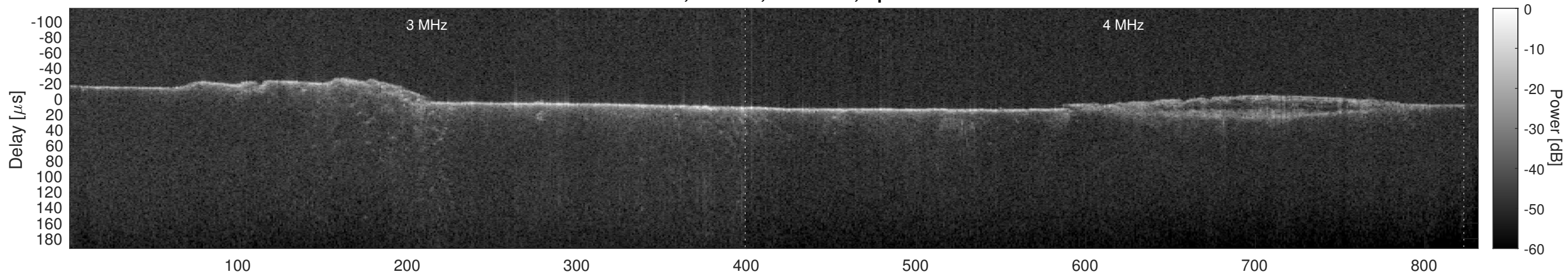
Orbit 5680, Cluttergram
