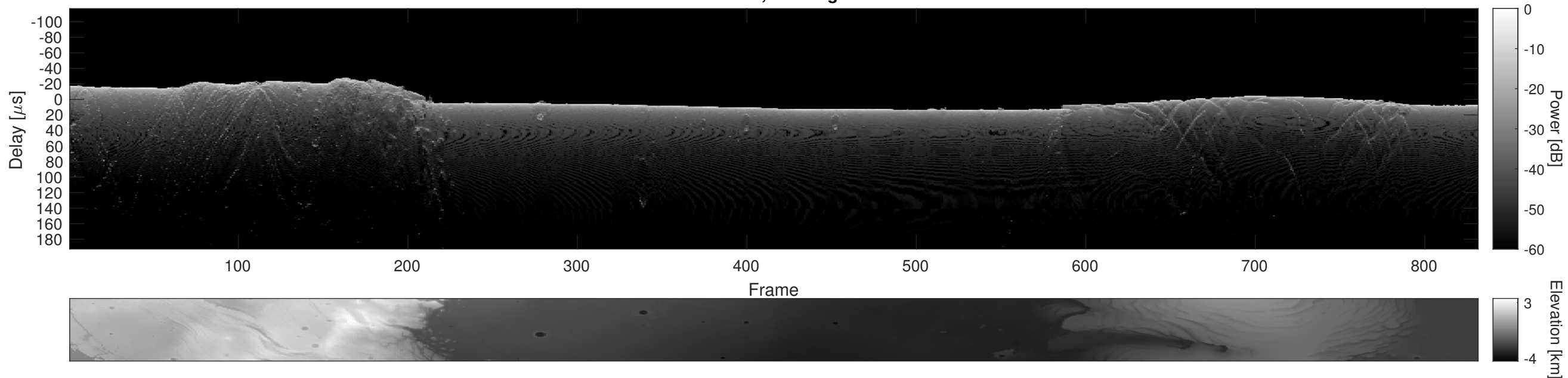
Orbit 5680, Cluttergram
