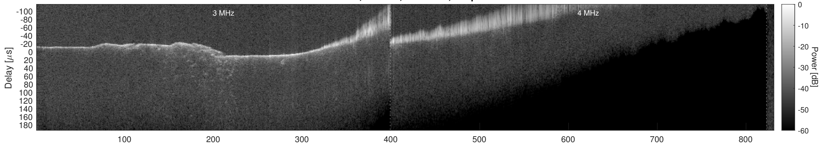
Orbit 5680, Window, Channel 2, Optimized
