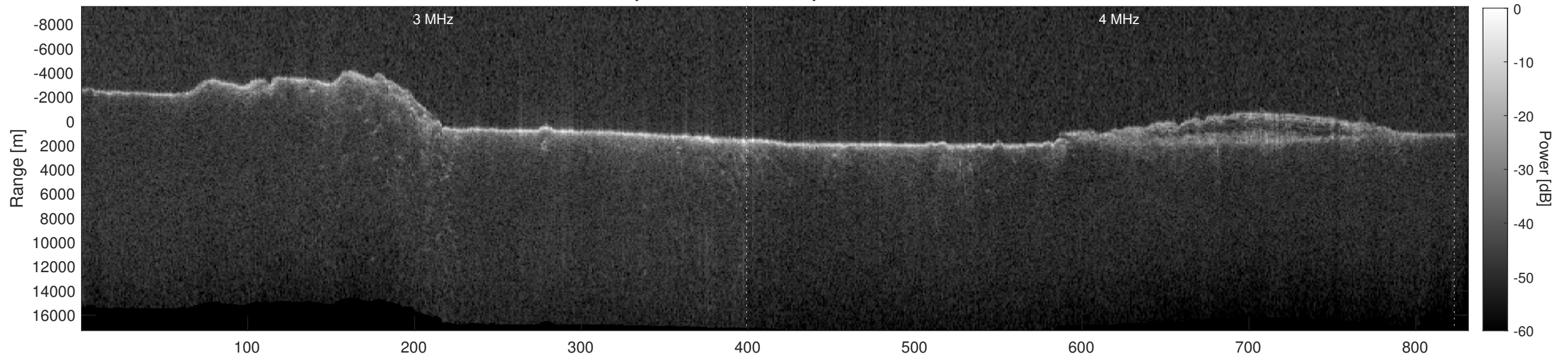
Orbit 5680, Depth-Corrected Cluttergram
