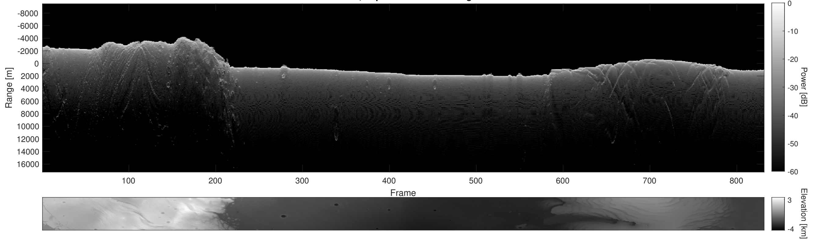
Orbit 5680, Depth-Corrected Cluttergram
