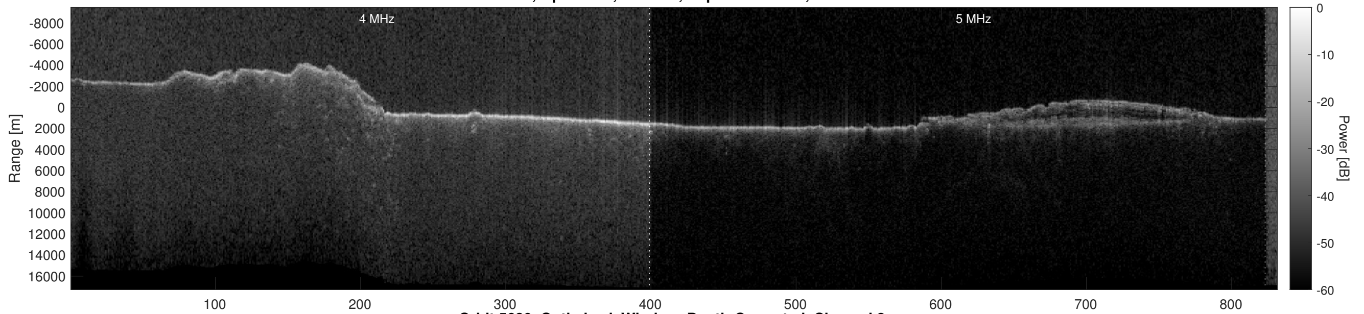
Orbit 5680, Optimized, Window, Depth-Corrected, Channel 2
