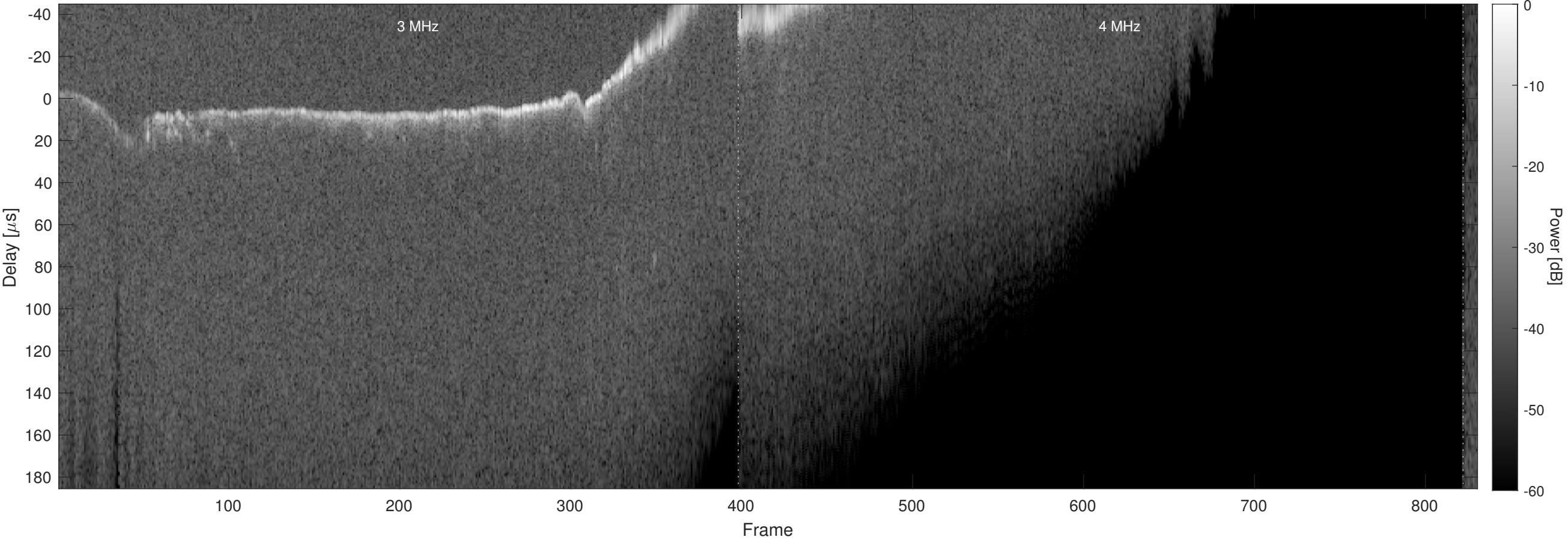
Orbit 5682, Chapman, Window, Channel 2
