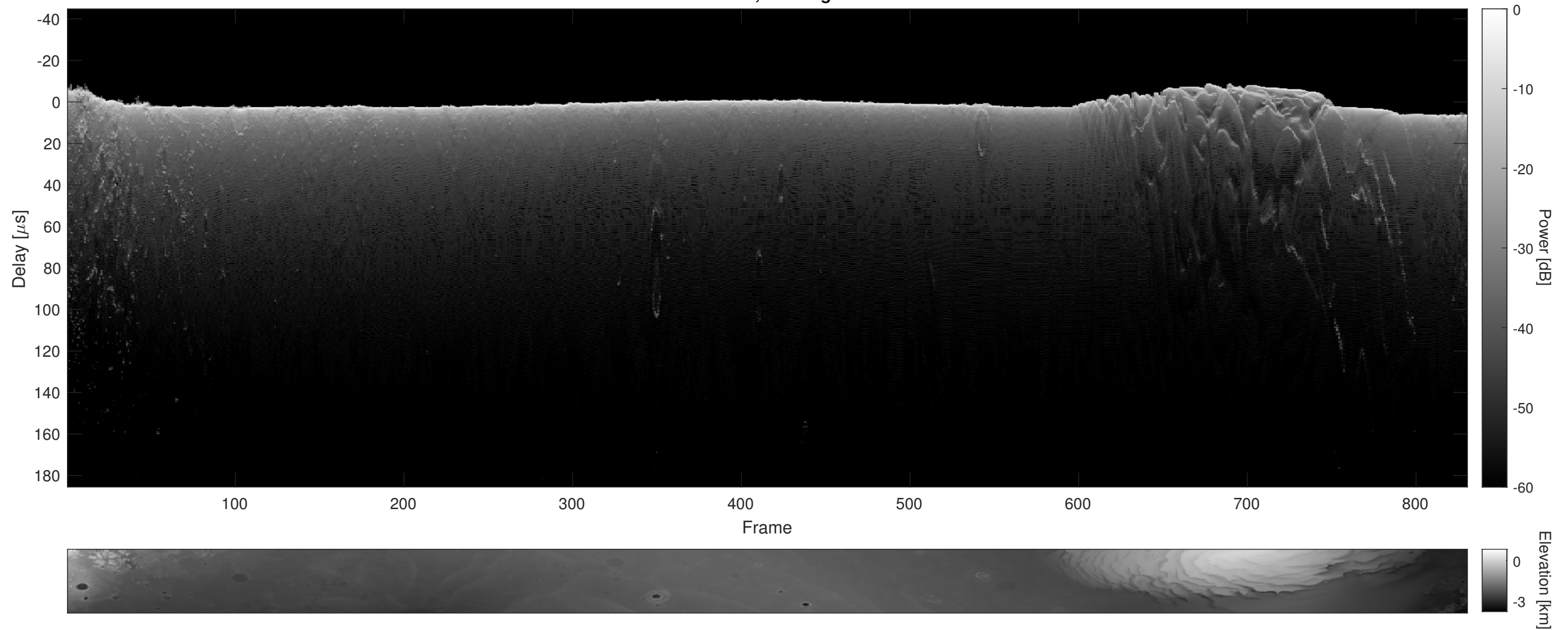
Orbit 5682, Cluttergram
