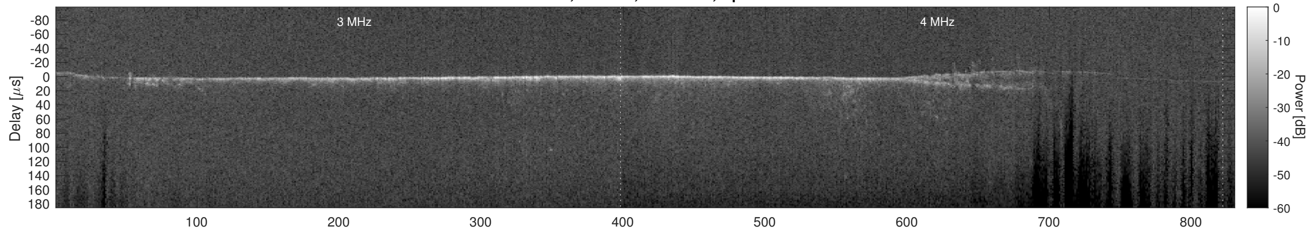
Orbit 5682, Cluttergram
