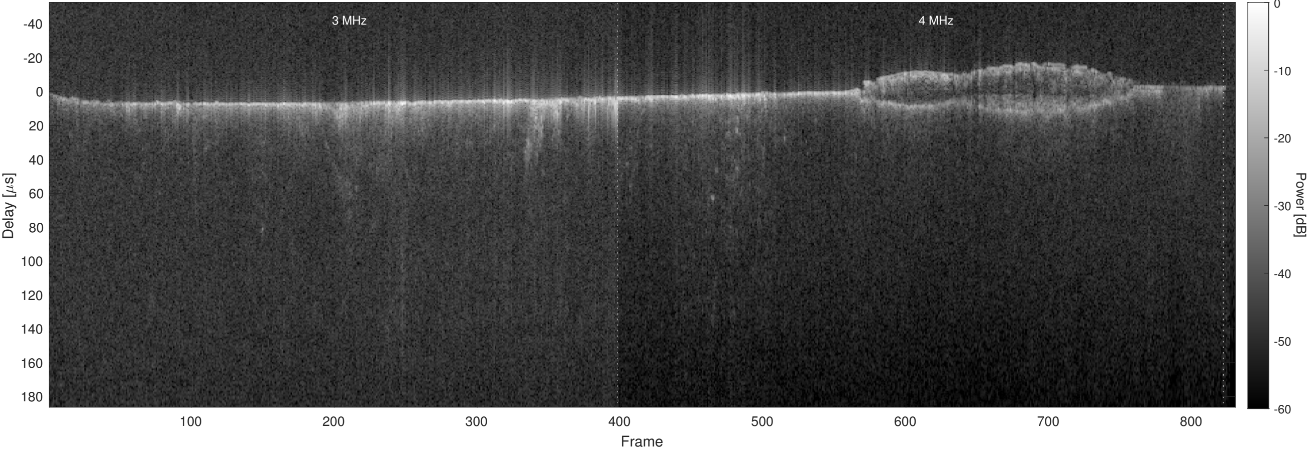
Orbit 5683, Optimized, No Window, Channel 2
