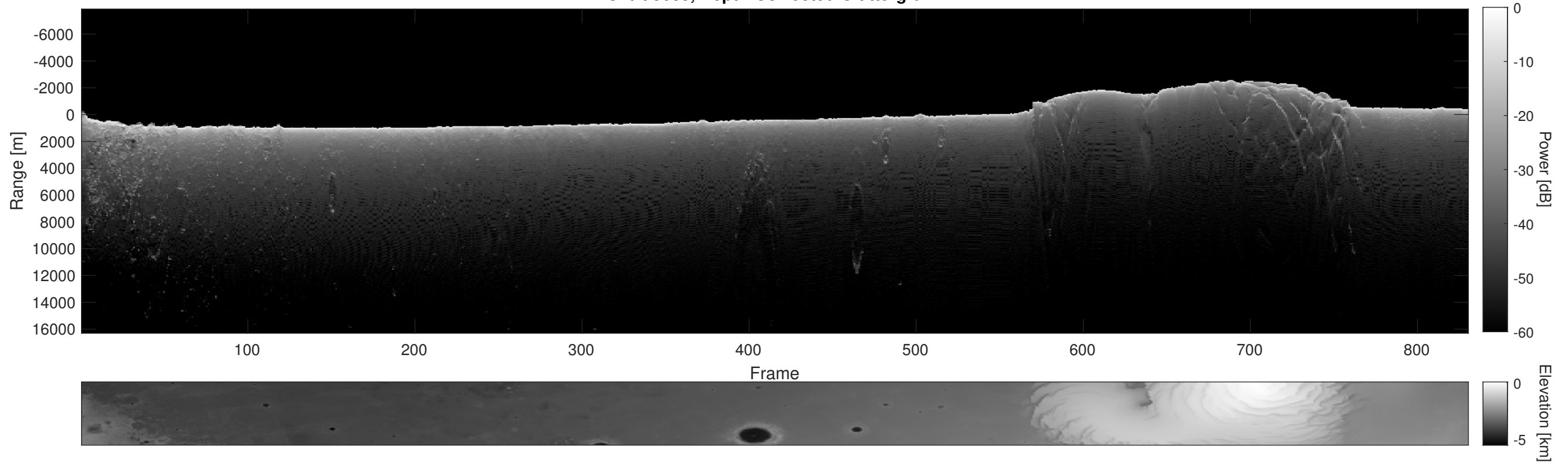
Orbit 5683, Depth-Corrected Cluttergram
