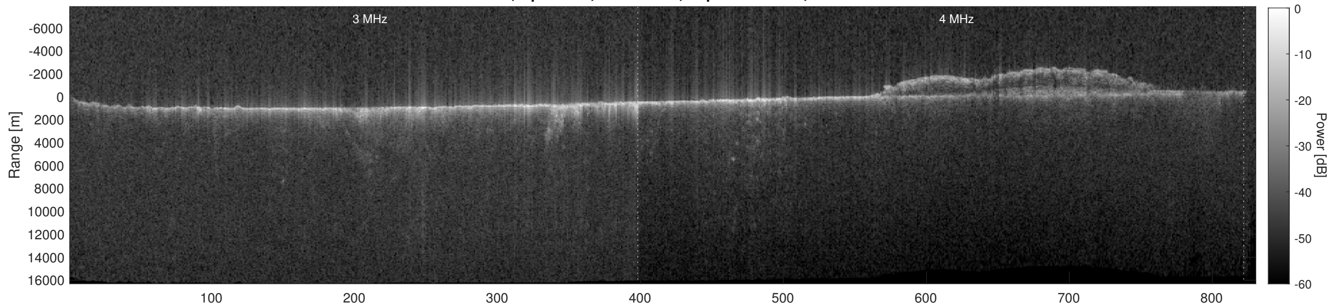
Orbit 5683, Depth-Corrected Cluttergram
