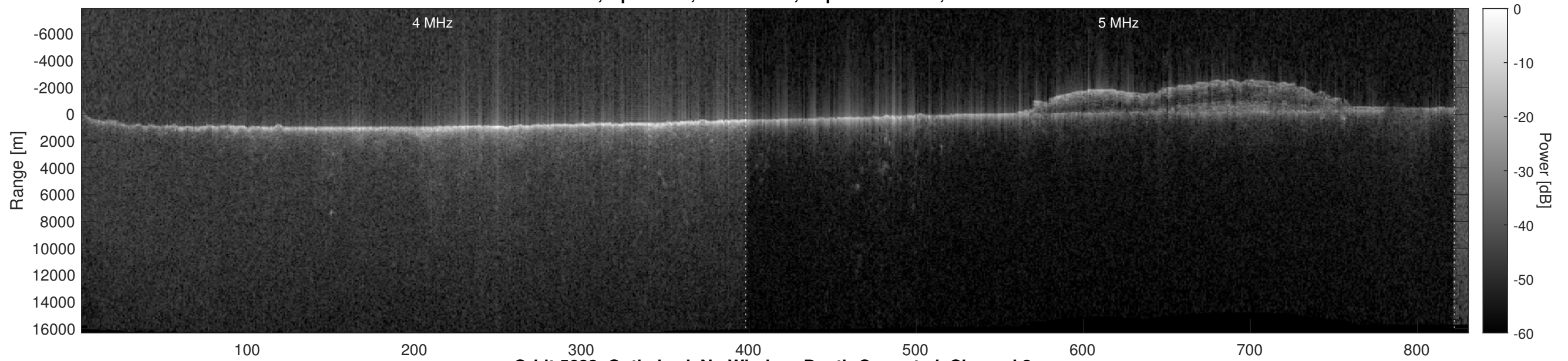
Orbit 5683, Optimized, No Window, Depth-Corrected, Channel 2
