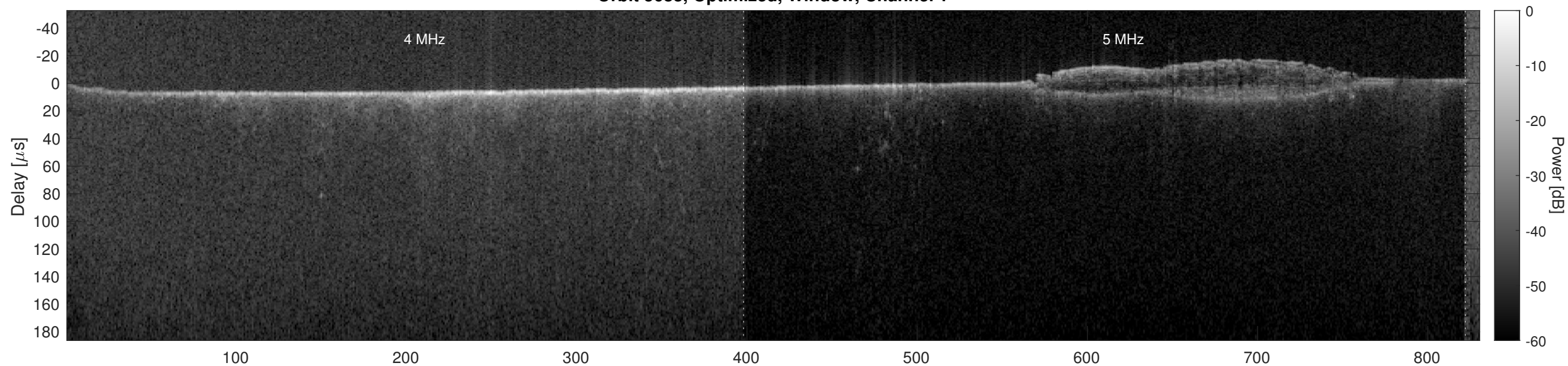
Orbit 5683, Optimized, Window, Channel 2
