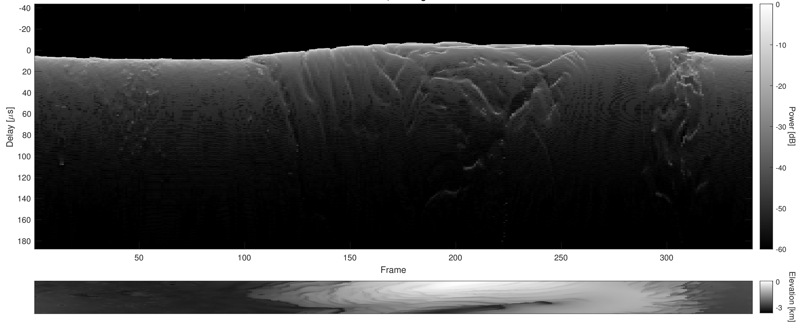
Orbit 5684, Cluttergram
