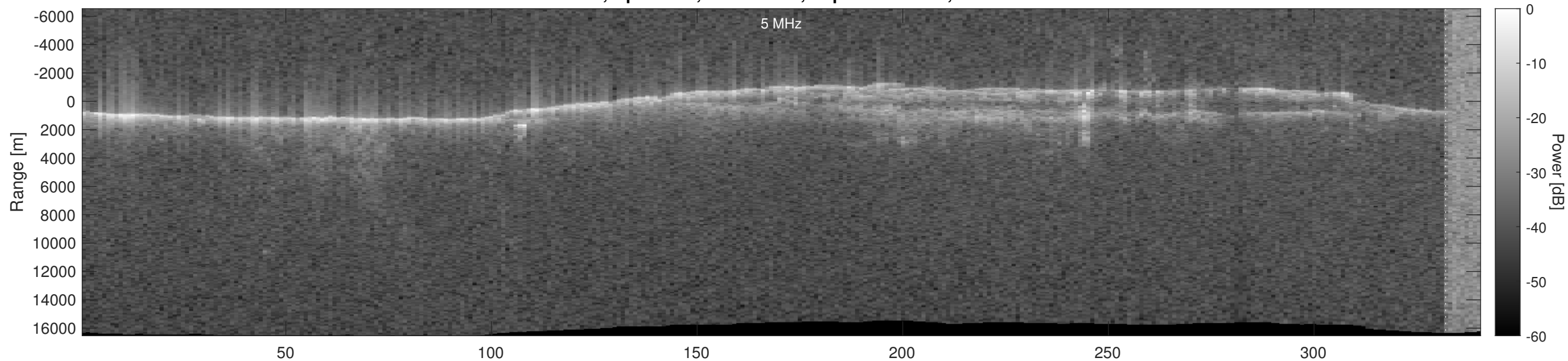
Orbit 5684, Optimized, No Window, Depth-Corrected, Channel 2
