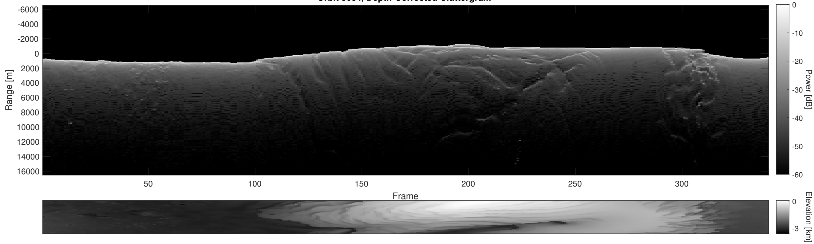
Orbit 5684, Depth-Corrected Cluttergram
