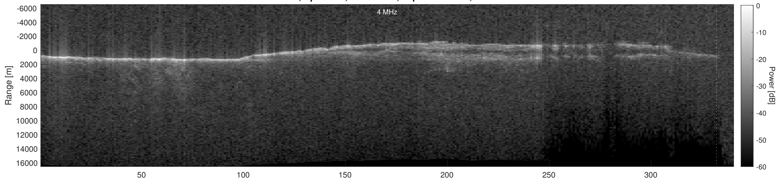
Orbit 5684, Depth-Corrected Cluttergram
