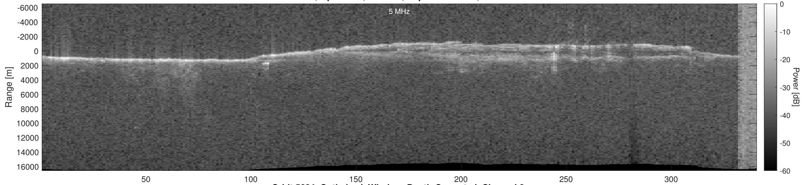
Orbit 5684, Optimized, Window, Depth-Corrected, Channel 2
