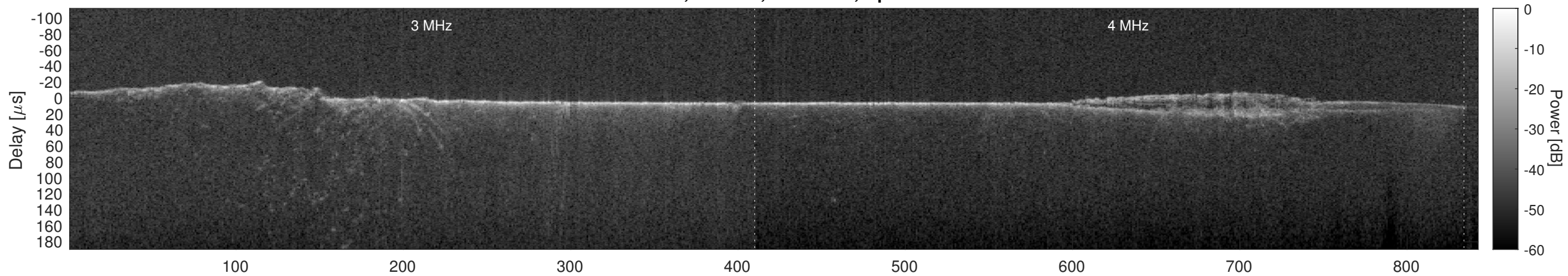
Orbit 5686, Cluttergram
