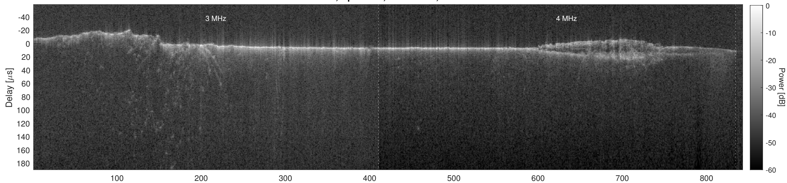
Orbit 5686, Cluttergram
