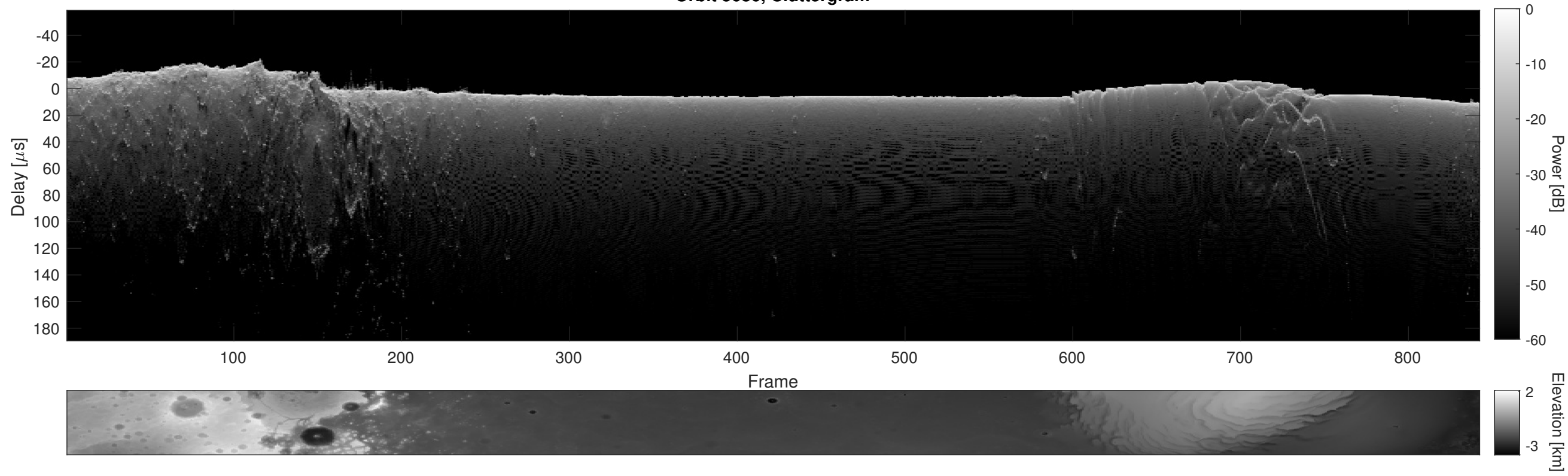
Orbit 5686, Cluttergram
