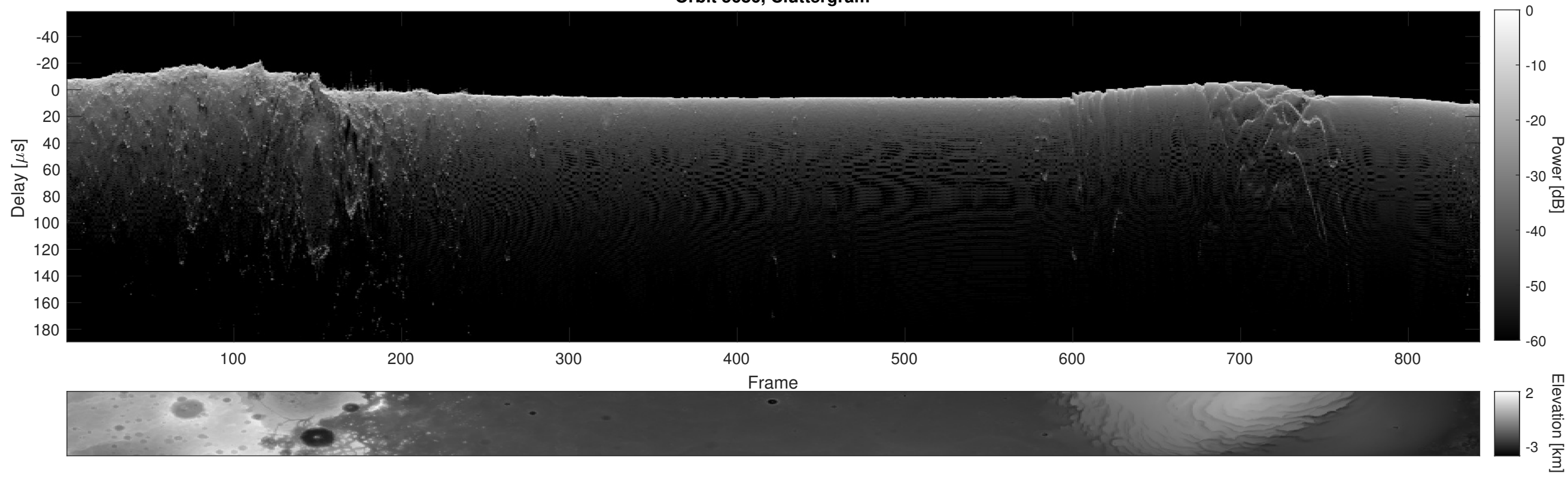
Orbit 5686, Cluttergram
