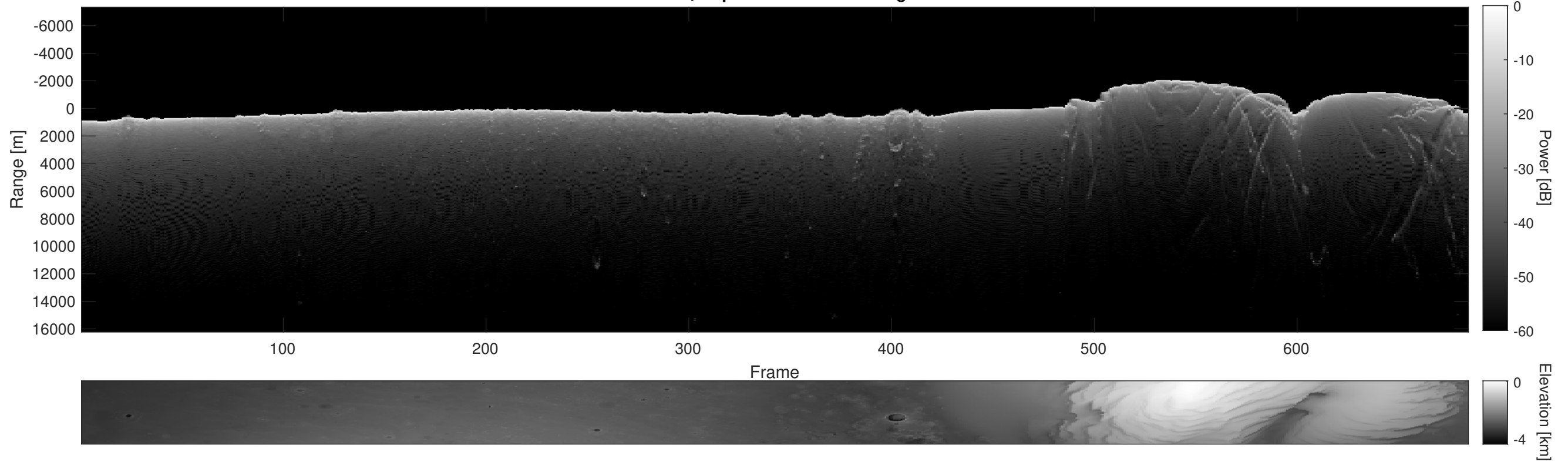
Orbit 5688, Depth-Corrected Cluttergram
