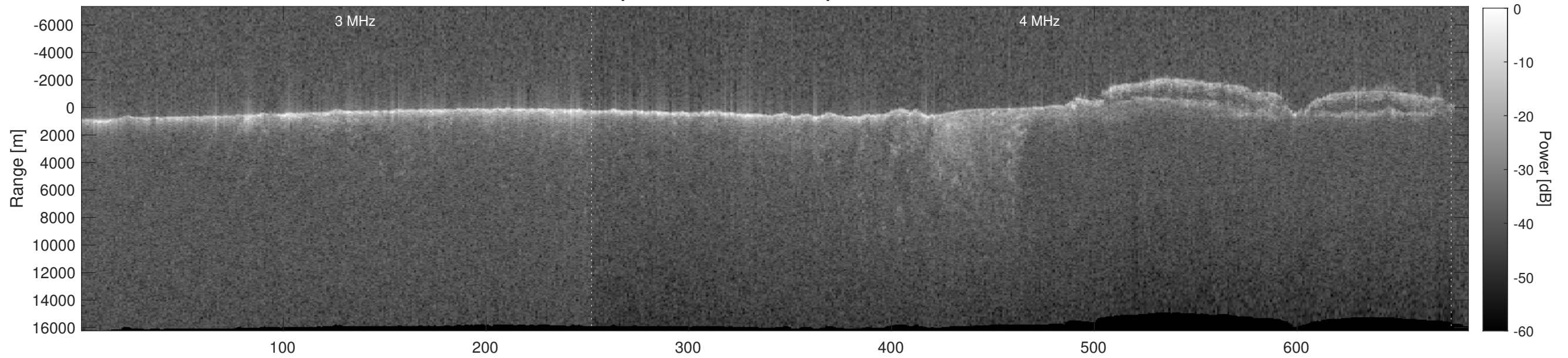
Orbit 5688, Depth-Corrected Cluttergram
