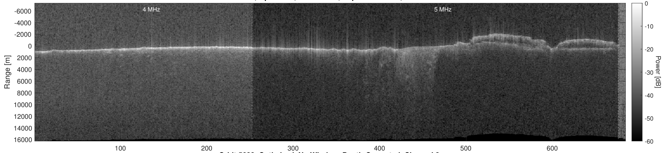
Orbit 5688, Optimized, No Window, Depth-Corrected, Channel 2
