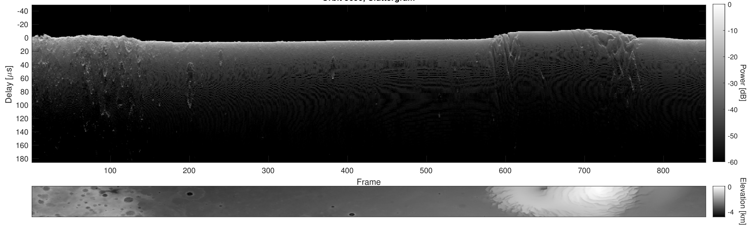
Orbit 5690, Cluttergram
