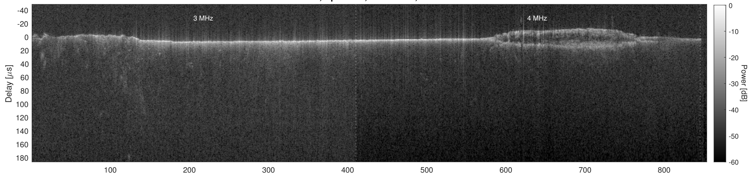
Orbit 5690, Cluttergram
