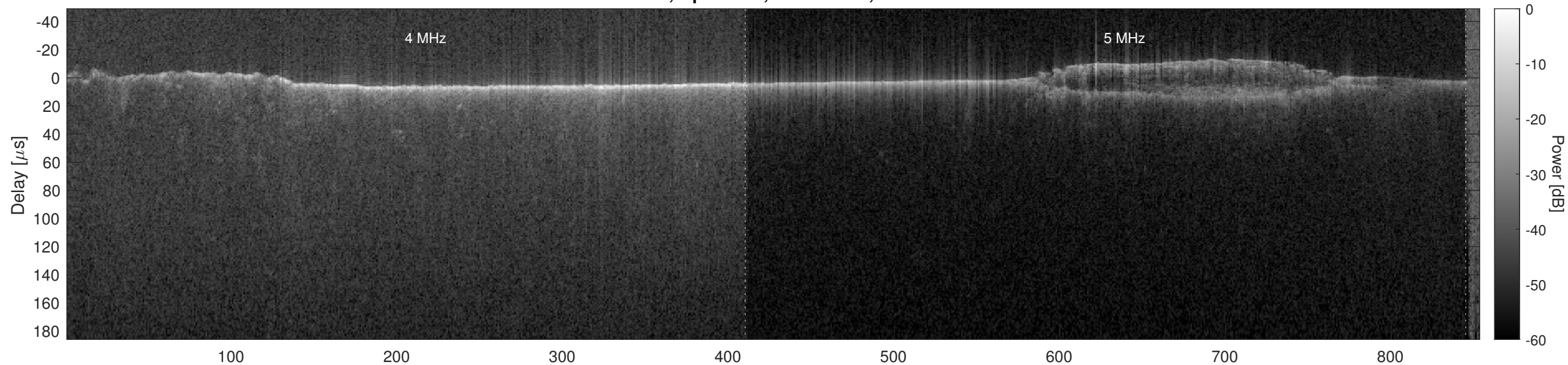
Orbit 5690, Optimized, No Window, Channel 2
