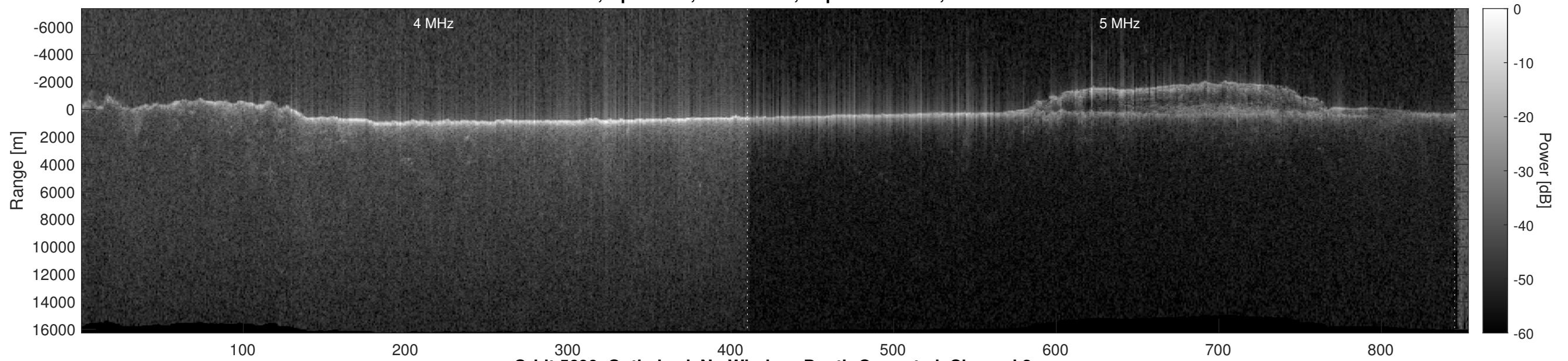
Orbit 5690, Optimized, No Window, Depth-Corrected, Channel 2
