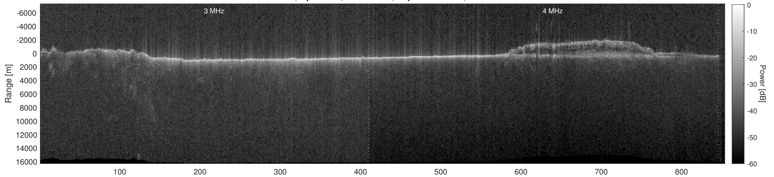
Orbit 5690, Depth-Corrected Cluttergram
