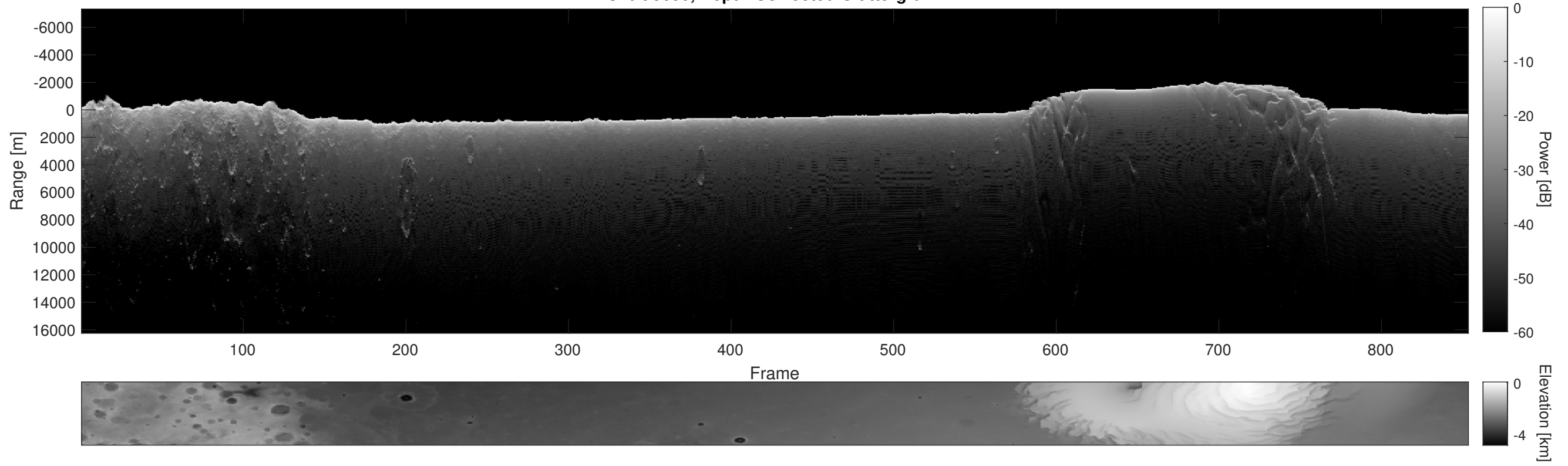
Orbit 5690, Depth-Corrected Cluttergram
