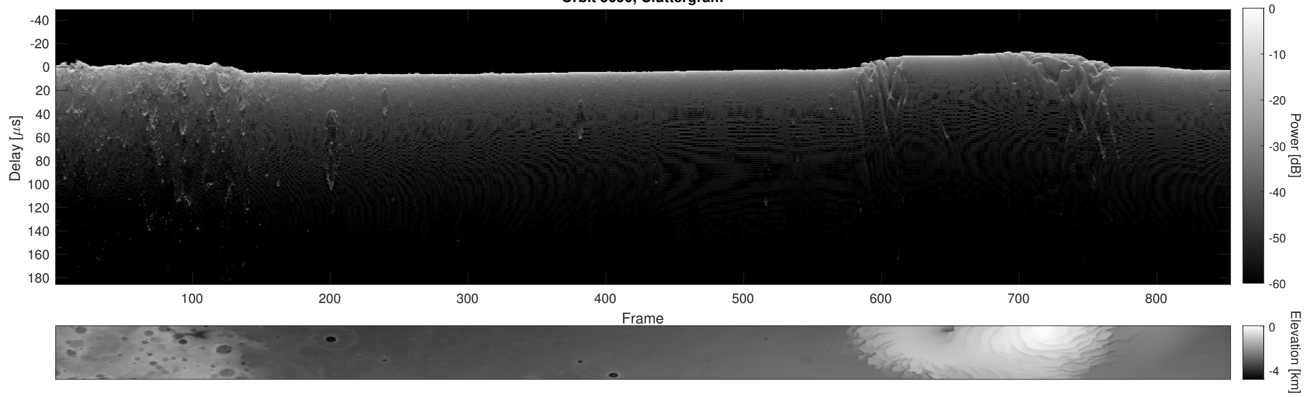
Orbit 5690, Cluttergram
