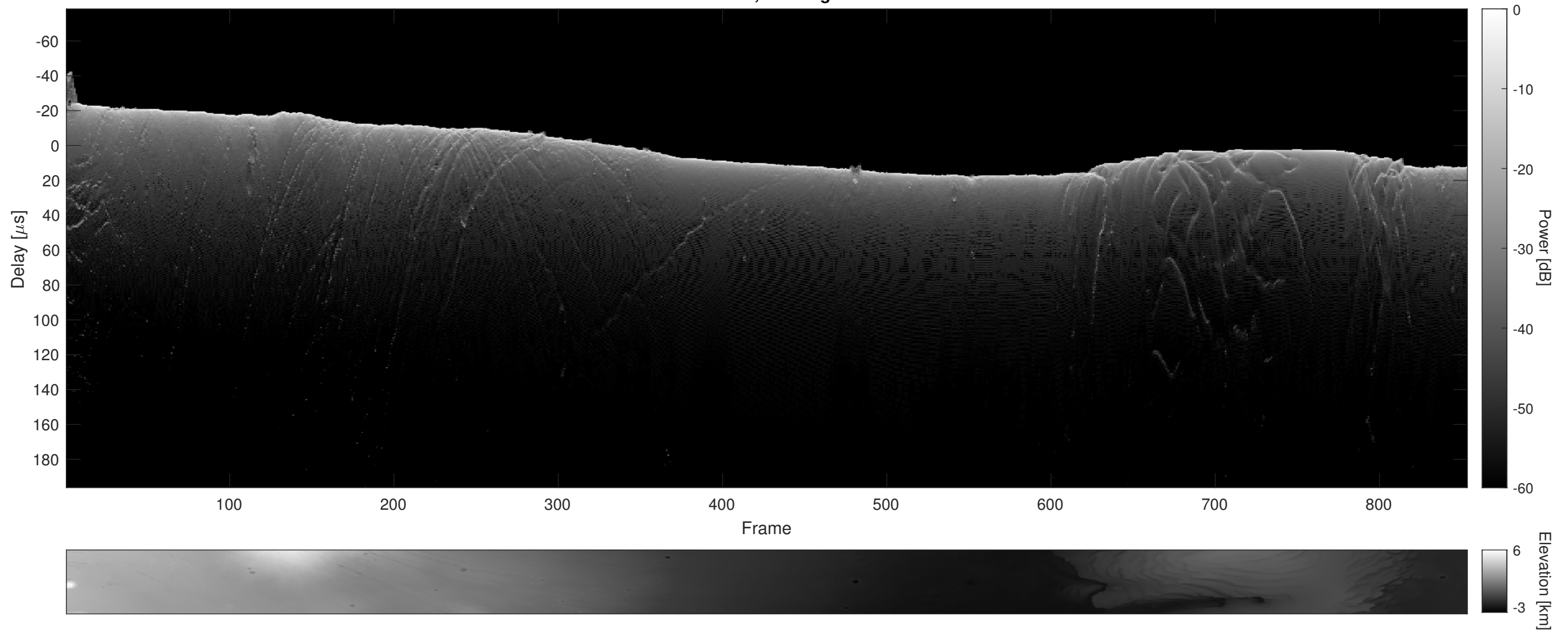
Orbit 5691, Cluttergram
