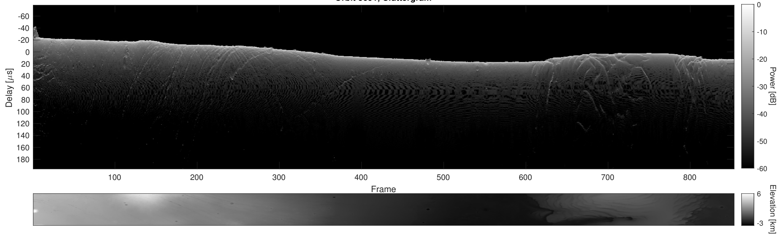
Orbit 5691, Cluttergram
