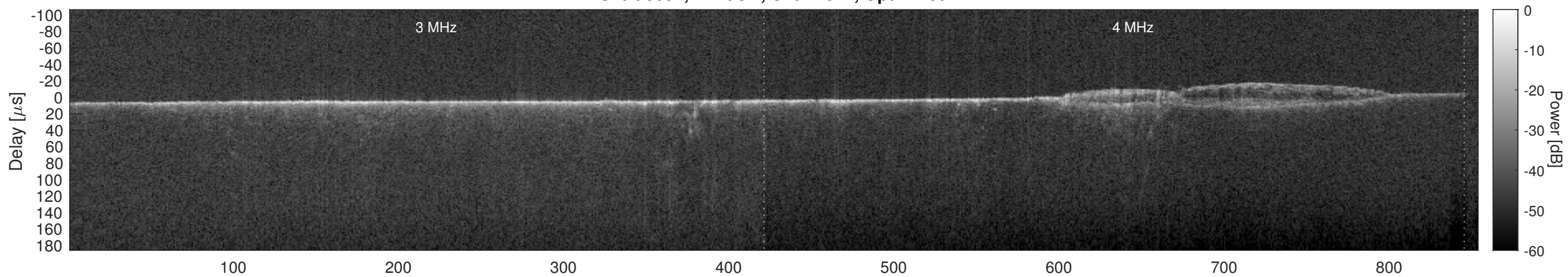
Orbit 5694, Cluttergram
