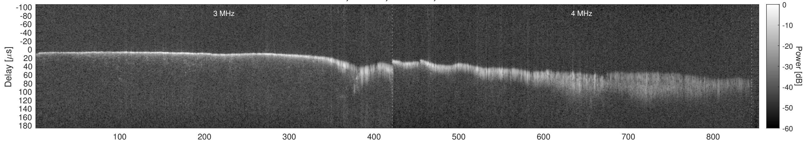
Orbit 5694, Window, Channel 2, Chapman
