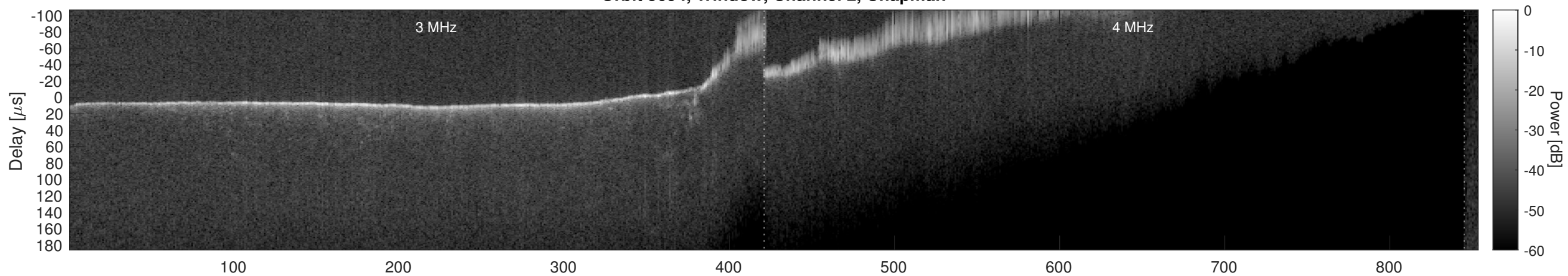
Orbit 5694, Window, Channel 2, Optimized
