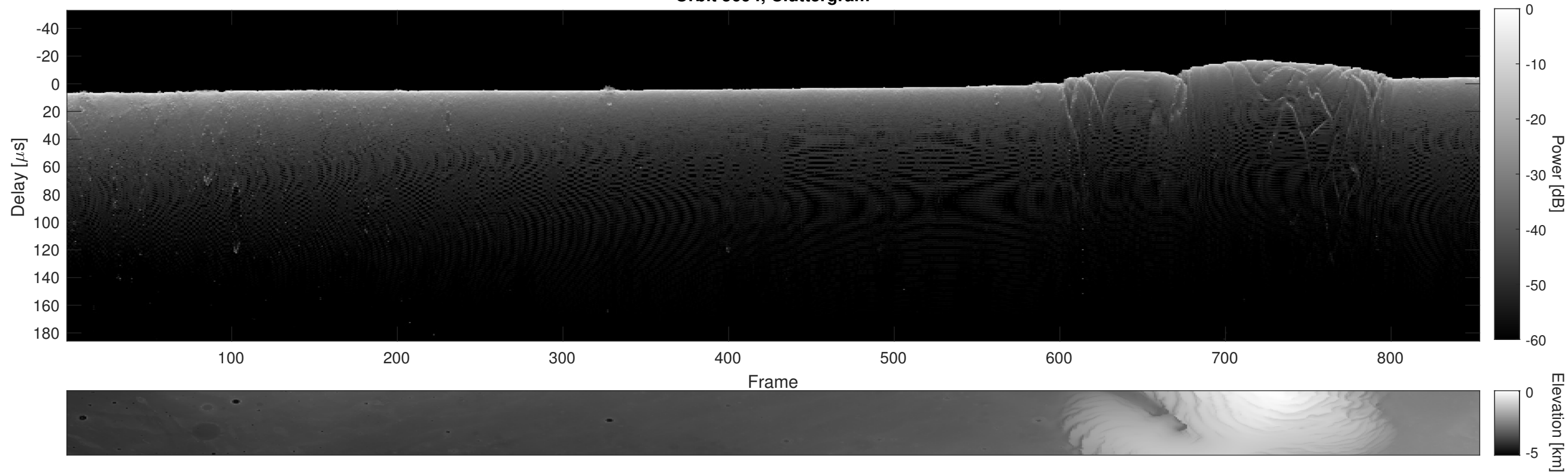
Orbit 5694, Cluttergram
