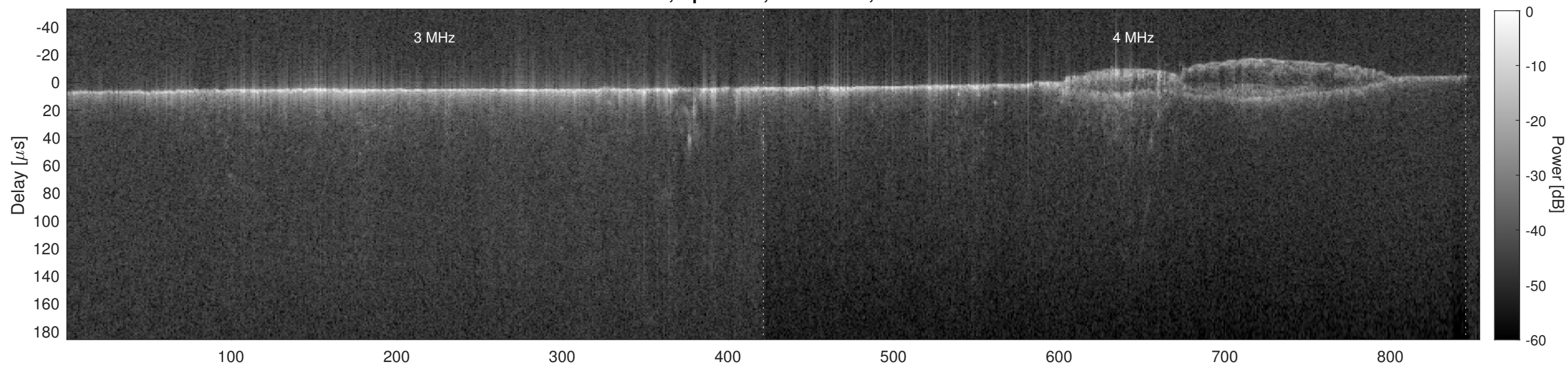
Orbit 5694, Cluttergram
