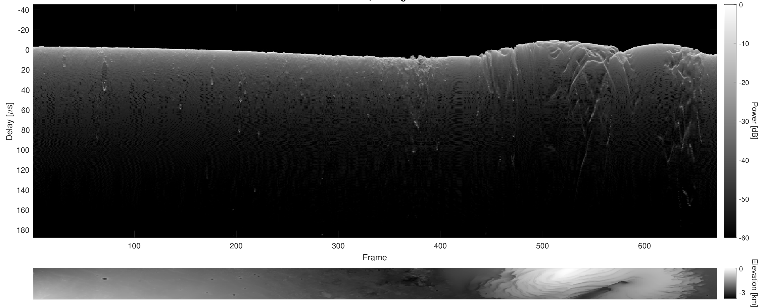
Orbit 5695, Cluttergram
