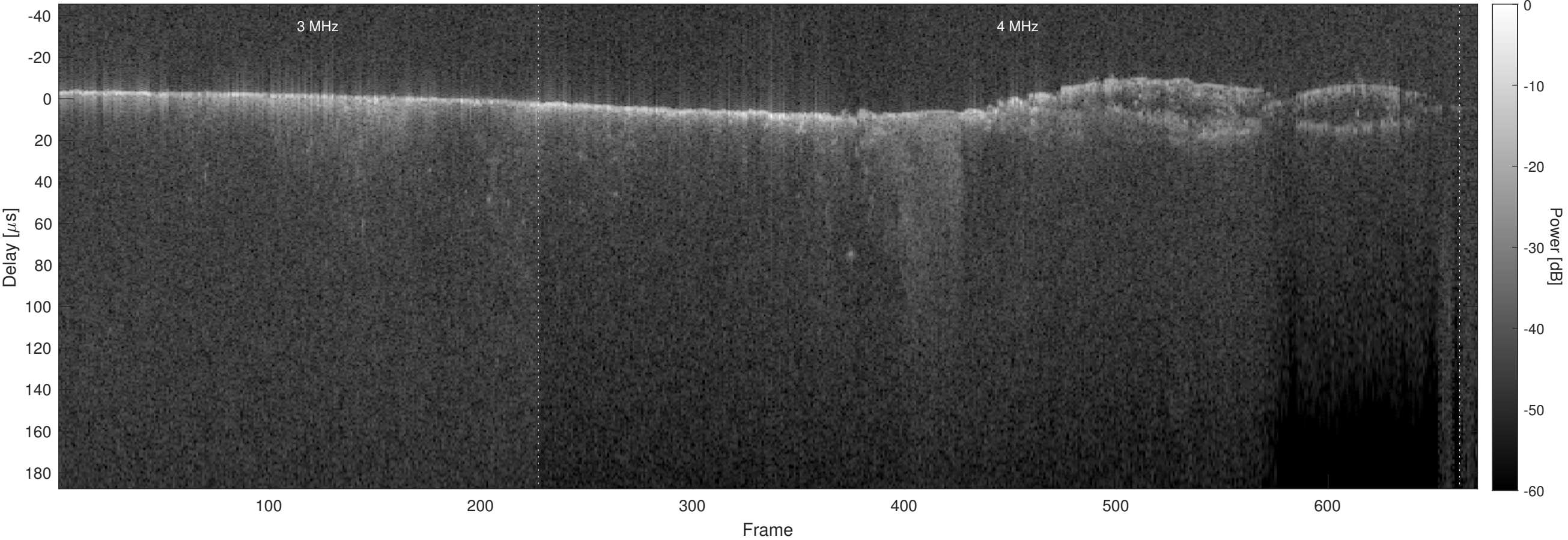
Orbit 5695, Optimized, No Window, Channel 2
