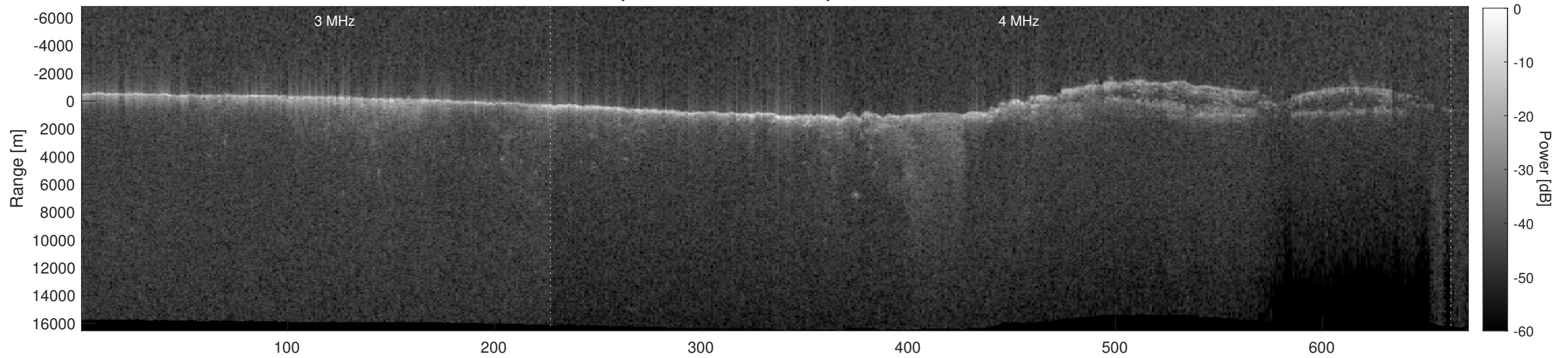
Orbit 5695, Depth-Corrected Cluttergram
