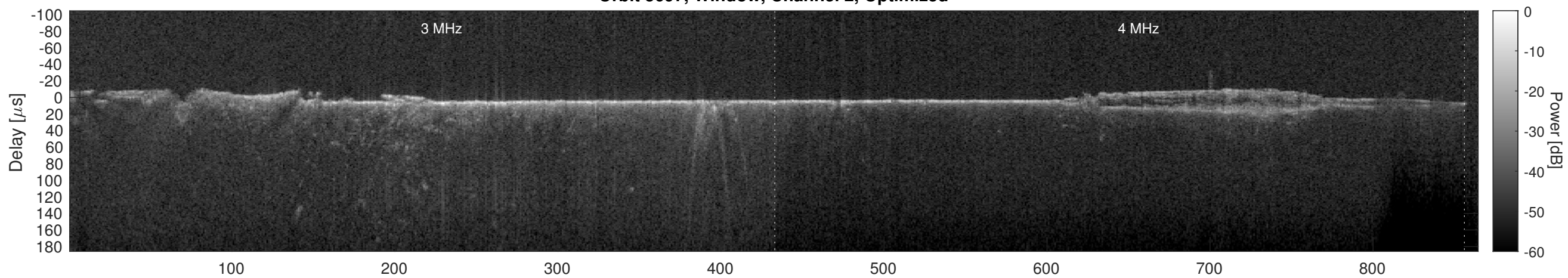
Orbit 5697, Cluttergram
