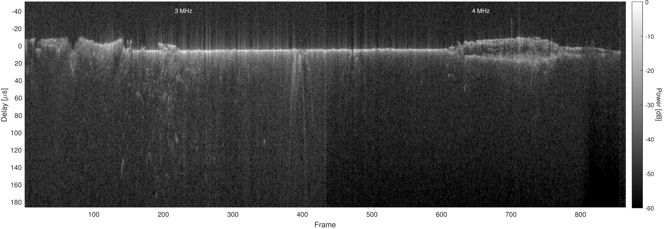
Orbit 5697, Optimized, No Window, Channel 2
