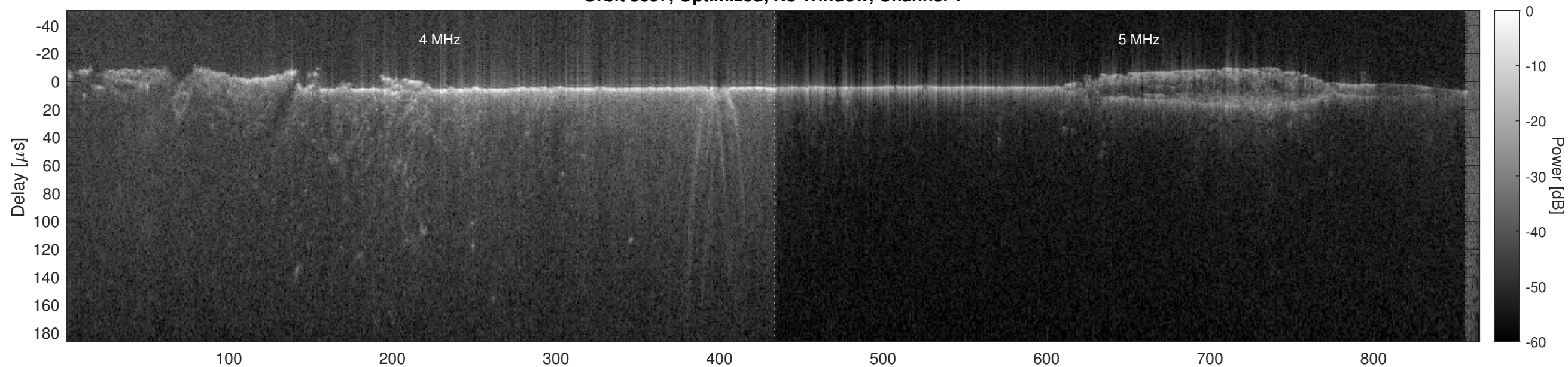
Orbit 5697, Optimized, No Window, Channel 2
