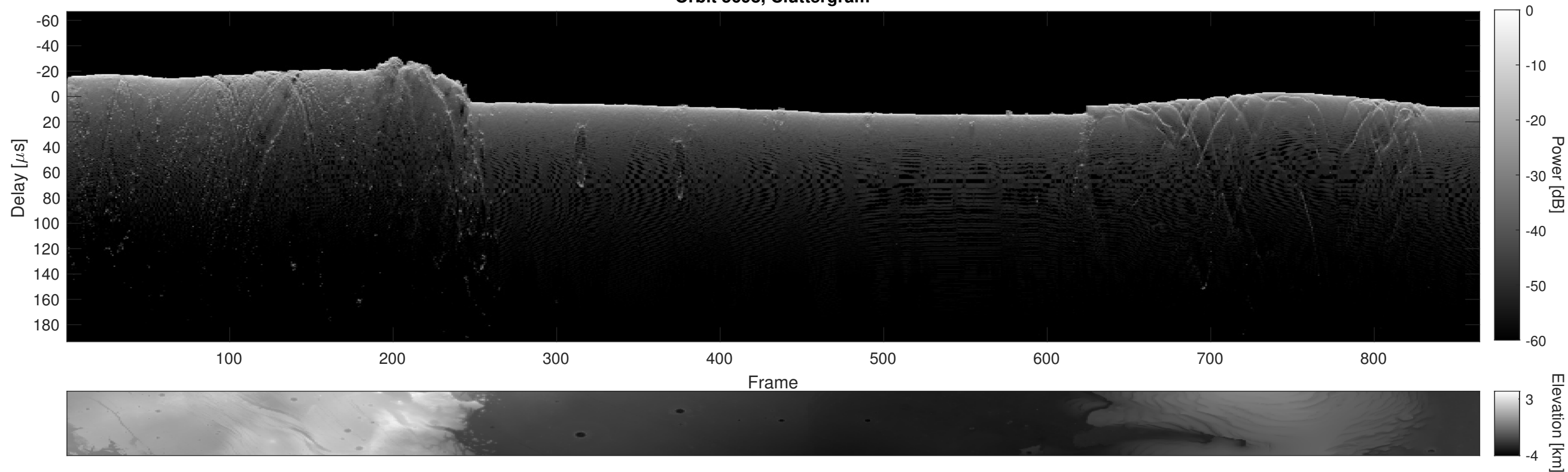
Orbit 5698, Cluttergram
