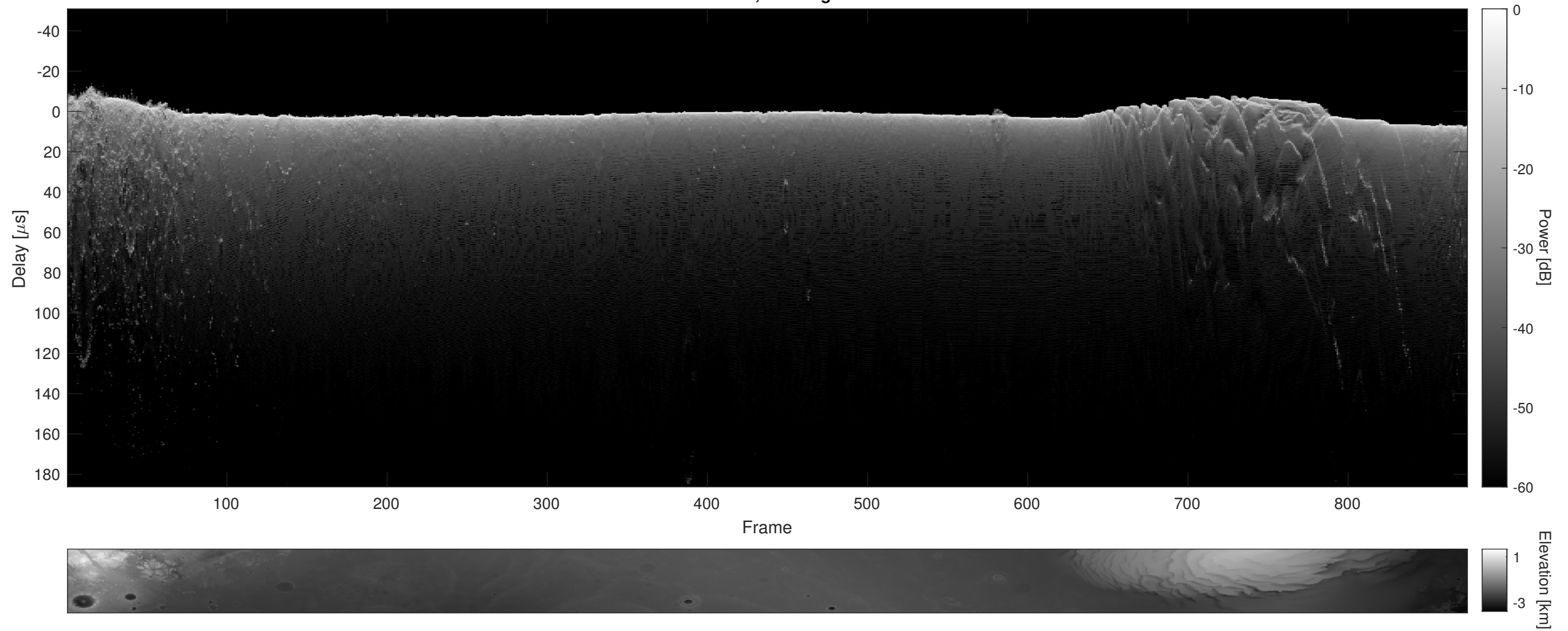
Orbit 5700, Cluttergram
