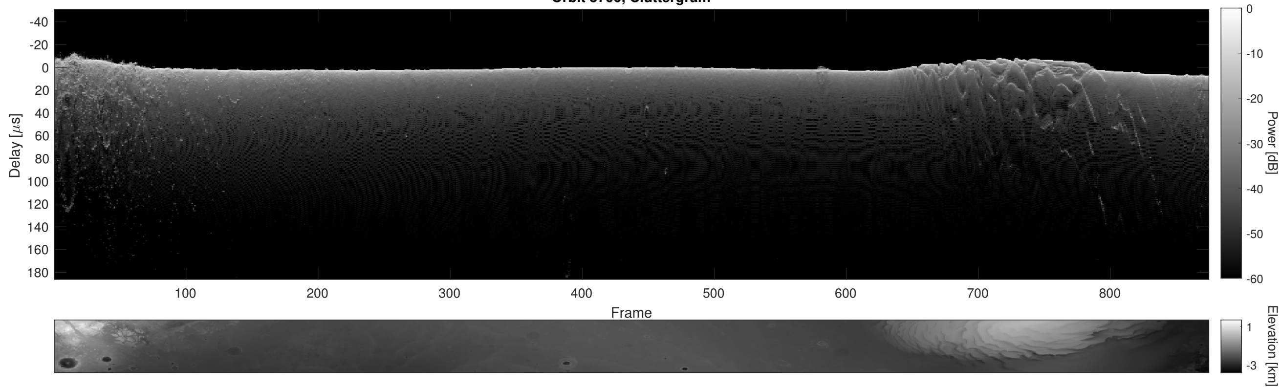
Orbit 5700, Cluttergram
