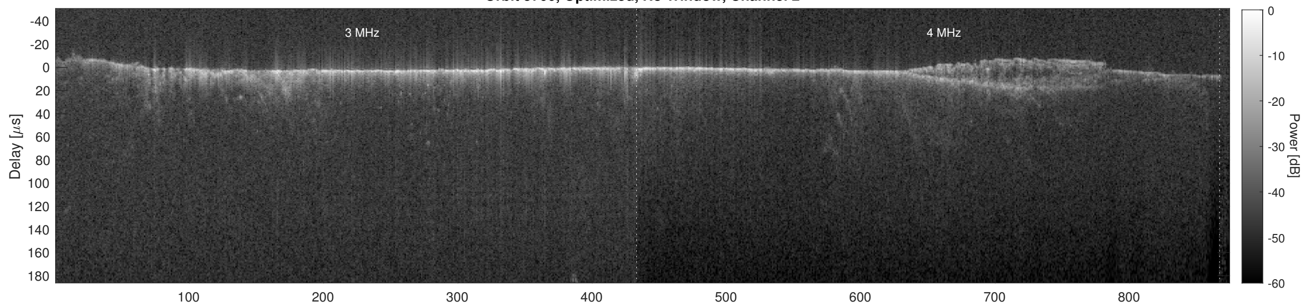
Orbit 5700, Cluttergram
