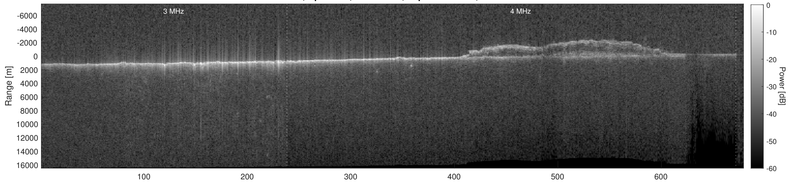
Orbit 5701, Depth-Corrected Cluttergram
