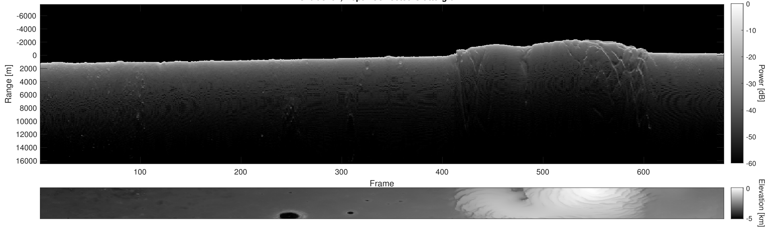
Orbit 5701, Depth-Corrected Cluttergram
