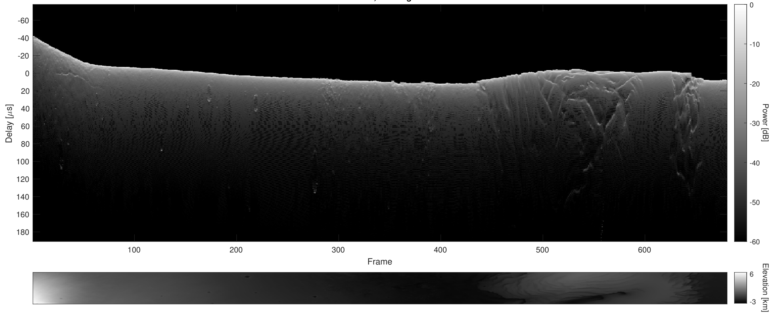
Orbit 5702, Cluttergram
