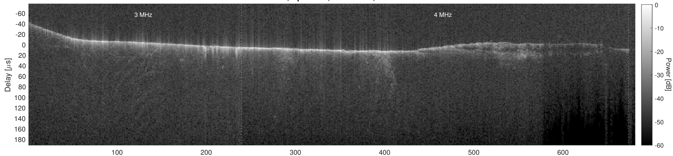
Orbit 5702, Cluttergram
