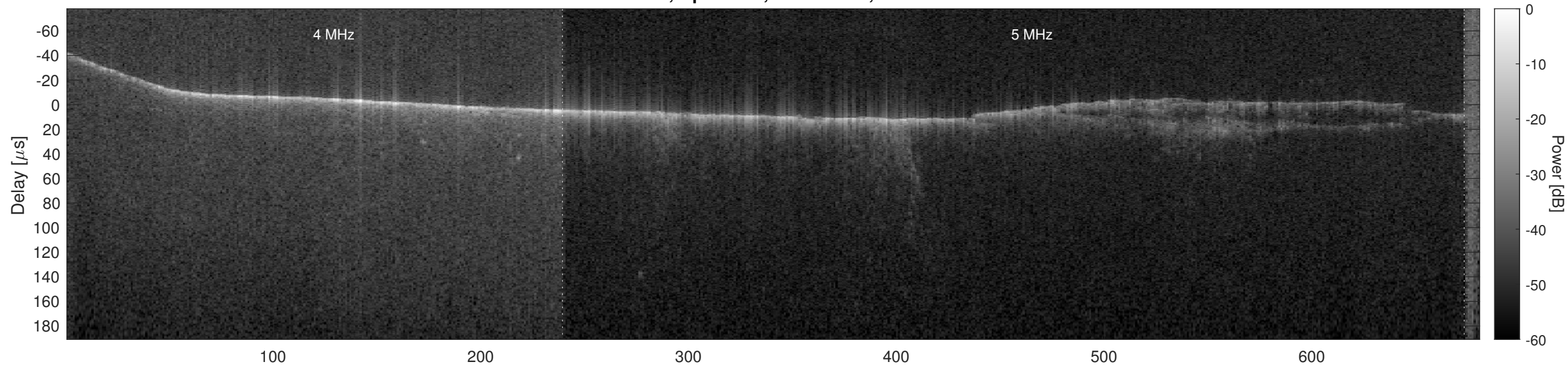
Orbit 5702, Optimized, No Window, Channel 2
