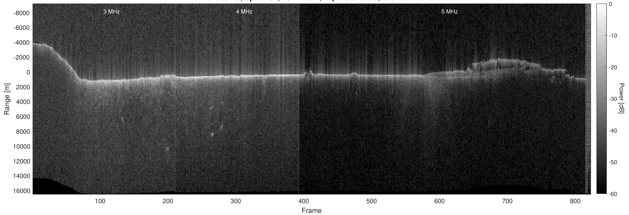
Orbit 5703, Optimized, No Window, Depth-Corrected, Channel 2
