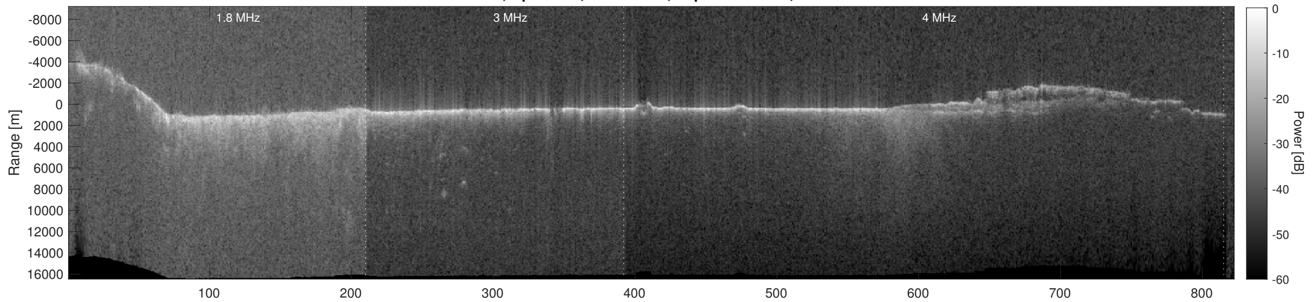
Orbit 5703, Depth-Corrected Cluttergram
