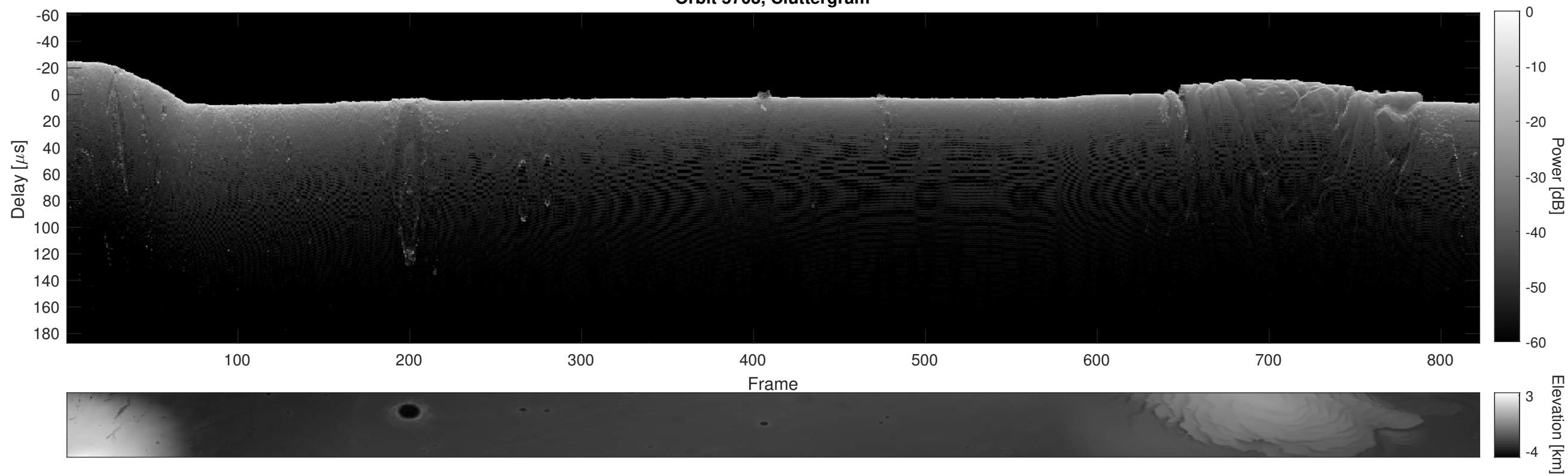
Orbit 5703, Cluttergram
