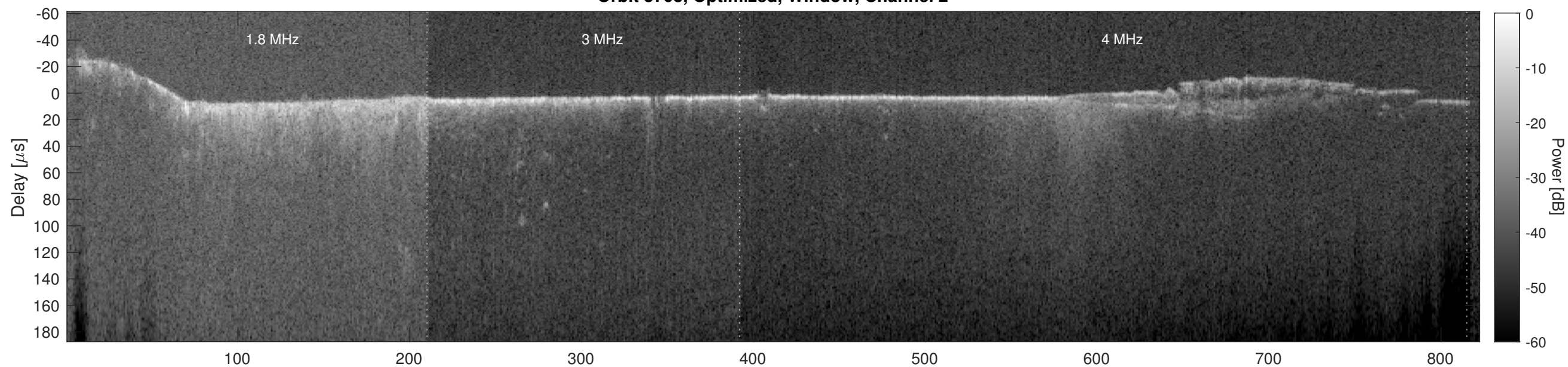
Orbit 5703, Cluttergram
